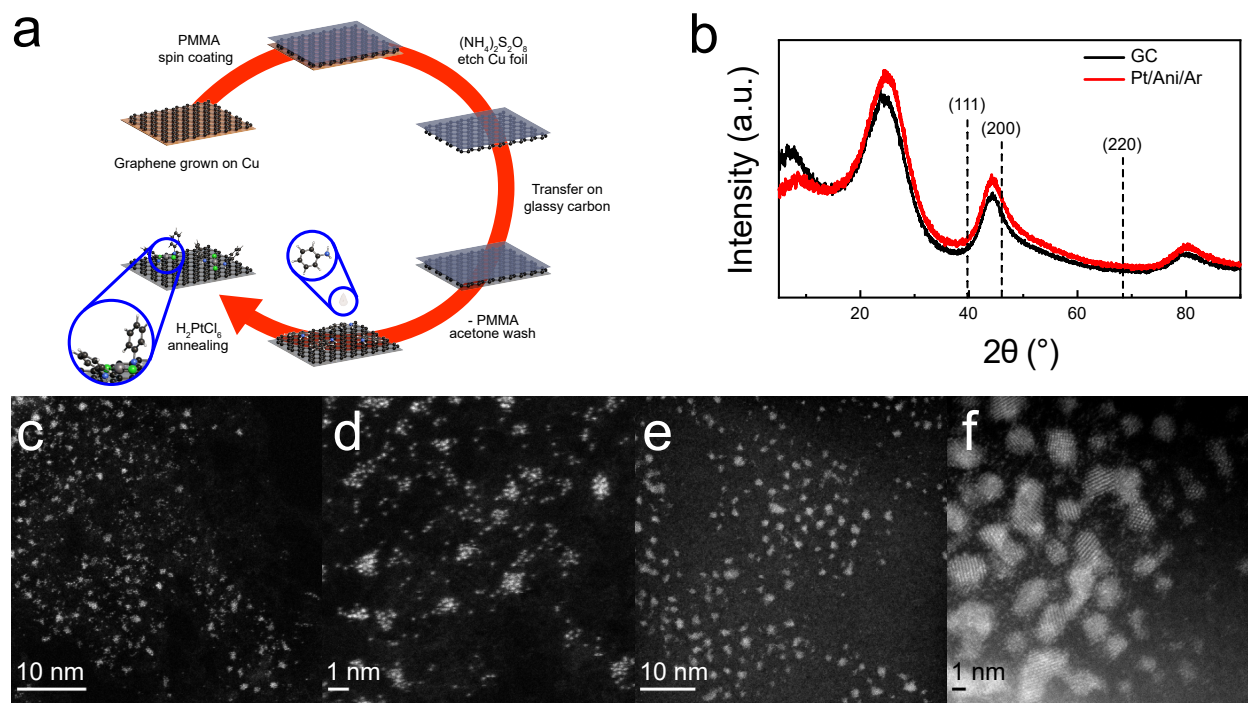
Figure 1. a , Schematic illustration of the synthesis process (5 steps) for Pt SSC (grey, Pt; green, Cl; blue, N; black, carbon; white, H). Step 1: graphene nanosheets are grown by chemical vapour deposition (CVD) on copper; Step 2: copper foil is etched after spin-coating with polymethyl methacrylate (PMMA) on top; Step 3: Thin-layer graphene coated with PMMA is then transferred onto a polished glassy carbon (GC) electrode; Step 4: after washing the PMMA with acetone and heating to 250 °C to remove trace organic contaminants, aniline is drop-cast onto the graphene-coated GC electrode and dried; Step 5: chloroplatinic acid in ethanol is then drop-cast and annealed under argon atmosphere. This sample is referred to as the (Pt/Ani/Ar) sample. The control sample (Pt/Ar) is prepared by the same method but without aniline. b , X-ray diffraction patterns for pristine GC and a (Pt/Ani/Ar) sample on GC; low magnification to high magnification atomic resolution HAADF-STEM images of (Pt/Ani/Ar) ( c , d ) and Pt/Ar ( e , f ).
