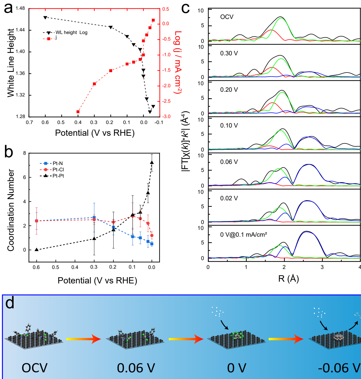
Figure 4. a , Amplitude of normalised white-line peak of Pt L_3 -edge operando XANES spectra (black) and the corresponding catalytic activity (red) at different potentials. \text{Log}(j) is calculated using relatively stable current density at the end of each CA test. b , Coordination number of Pt-N, Pt-Cl and Pt-Pt fitting paths for operando EXAFS data of Pt single-site complex at selected potentials by 0 V. Error bars in (b) represent the uncertainties of fitting results. c , Contribution of different paths (Pt-N, Pt-Cl and Pt-Pt) to fit the corresponding EXAFS spectra. The details of the fitting results shown in K-space and R-space can be found in Supplementary Figure S11. d , Proposed schematic model for the evolution of (Pt/Ani/Ar) sample from single-site complex to subnanoclusters based on the operando EXAFS analysis (grey, Pt; green, Cl; blue, N; black, carbon; white, H).
