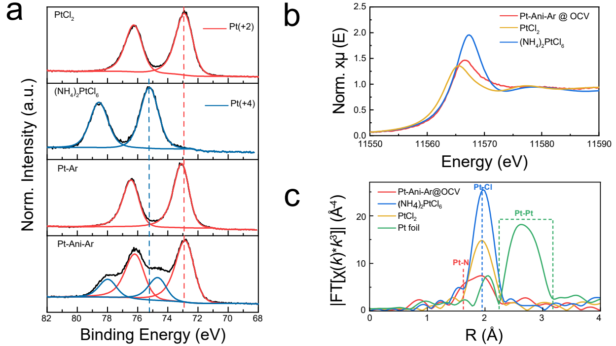
Figure 2. XPS spectra of Pt 4f (a) and XANES spectra (b) recorded at Pt L 3 -edge for the synthesised Pt SSC and control sample (Pt/Ar) compared with reference standards in the oxidation states of platinum(II) and platinum(IV). The vertical dashed red and blue lines in (a) indicate the peak positions of Pt 7/2 at the oxidation state of platinum(II) and platinum(IV). c, Corresponding k^3 -weighted Fourier-transformed Pt L 3 -edge EXAFS spectra of samples in (b) and standard Pt foil. The vertical dashed lines or area show the positions of Pt-N (red), Pt-Cl (blue), and Pt-Pt (green) peaks.
