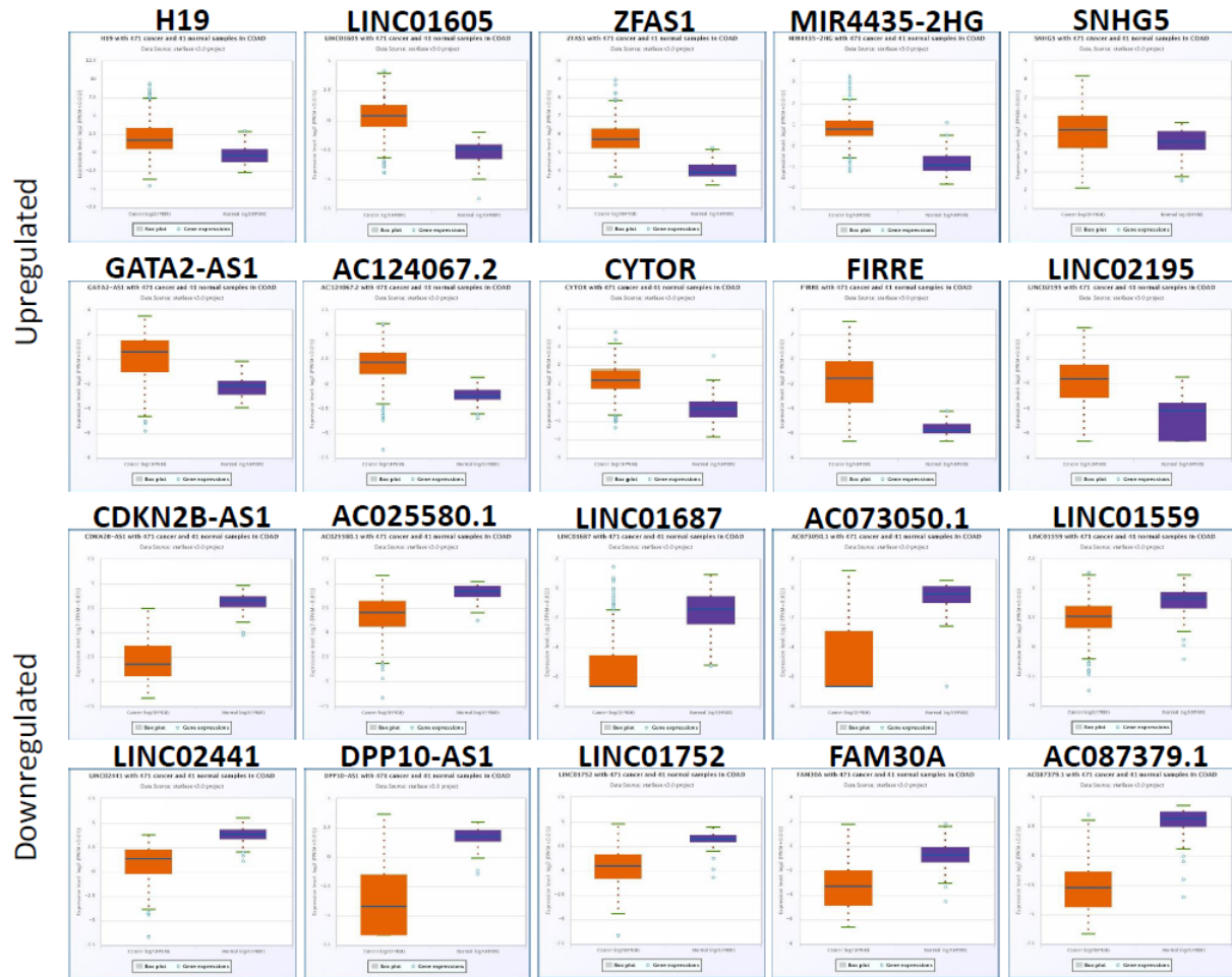
Supplementary figure 2. Expression of top 10 upregulated and top 10 downregulated lncRNAs in the TCGA COAD database. Expression of the indicated gene in COAD (n=471) compared to normal tissue (n=41) is shown as box plot. Data were retrieved from the starBase V3.0 database.
