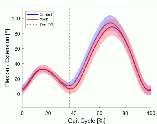
Figure 2: Sagittal plane knee ensemble average kinematic waveform across the gait cycle.
