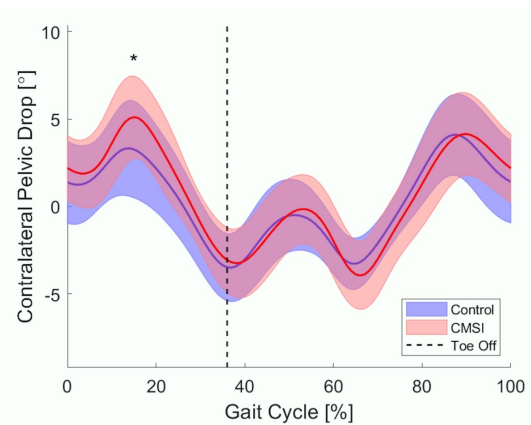
Figure 1: Frontal plane pelvis ensemble average kinematic waveform across the gait cycle.
