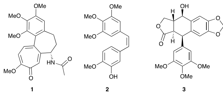
Figure 1. Structure of natural ligands that bind at the colchicine site of tubulin.
