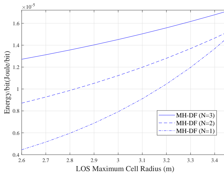
Figure 10. Energy-per-bit performance of the multi-hop system.
