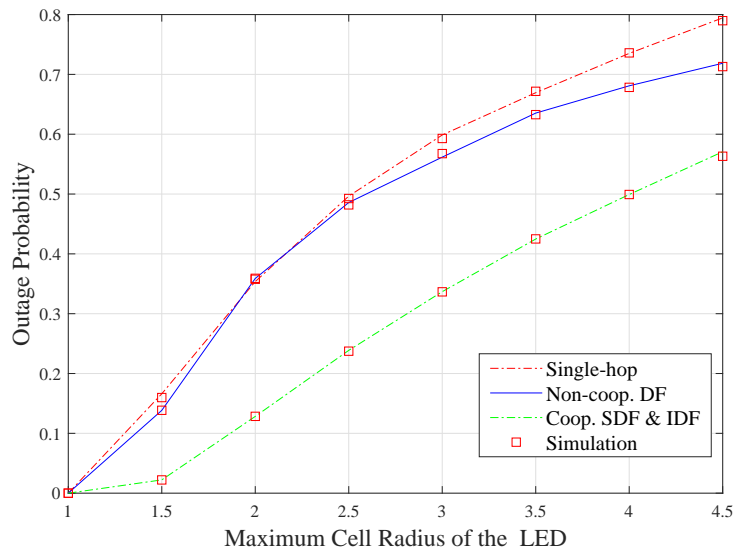
Figure 7. Performance comparison between the different VLC system setups as a function of VLC cell radius.
