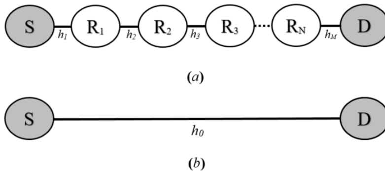
Figure 3. Basic block diagrams of the proposed VLC systems, (a) with N intermediate VLC relays and (b) with a direct VLC link.
