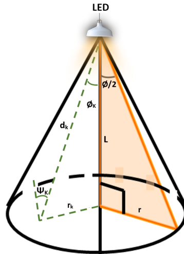
Figure 2. The line-of-sight channel of the VLC.
