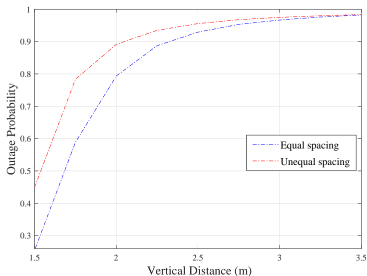
Figure 6. Simulated results of DF relay with N = 3 .
