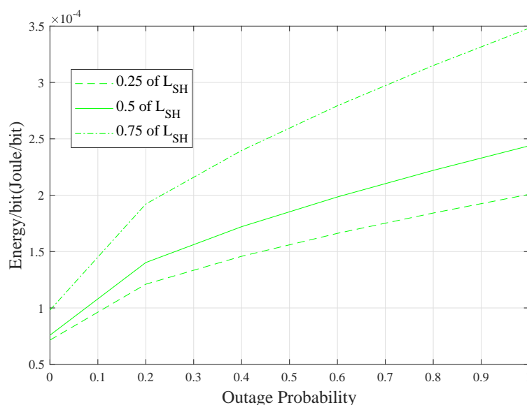
Figure 11. Energy consumption of the SDF system with respect to outage probability.
