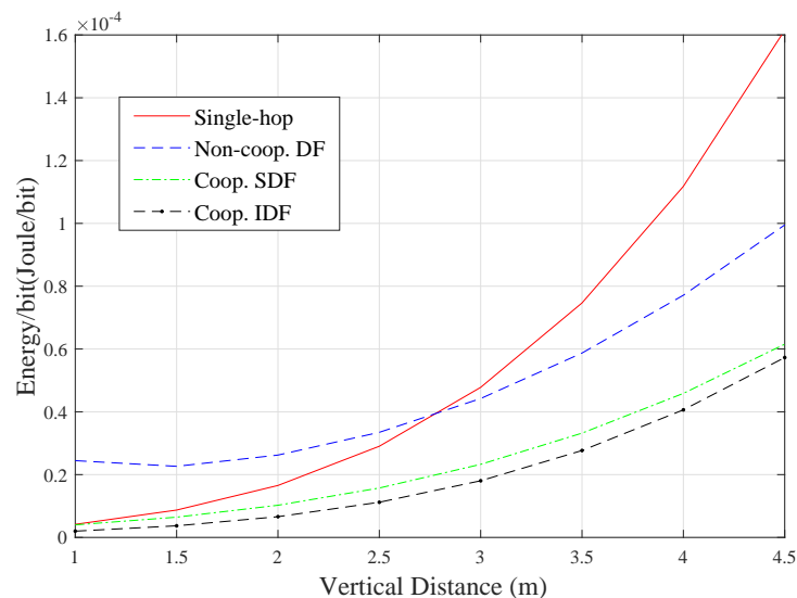
Figure 9. Energy performance comparison between the different VLC system setups.
