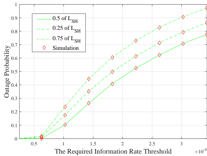
Figure 8. Average outage probability performance of the cooperative configurations as a function of the required information rate threshold values.
