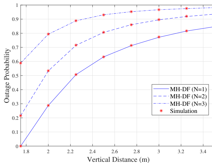
Figure 5. Outage probability of DF multi-hop scenarios (for N = 1, 2 and 3 ).
