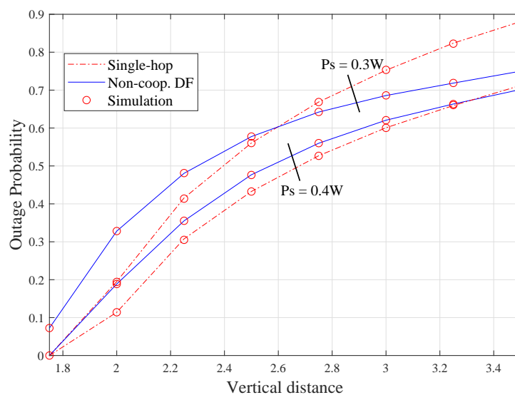
Figure 4. Outage probability of single-hop and non-cooperative DF relay configurations.
