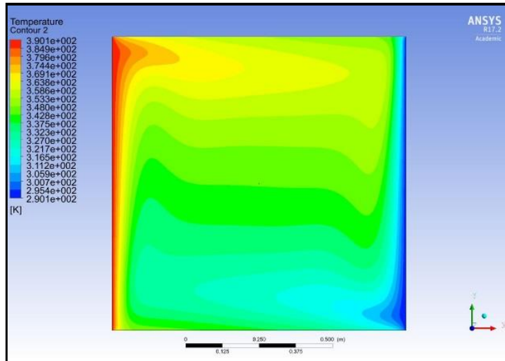
Fig 8a. Isotherms for silver-water nanofluid, Ra = 10^6 , P1 radiative flux with \Phi = 0.04 .
