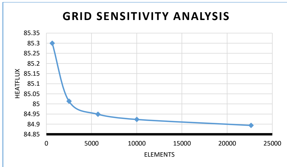
Fig 3: Mesh independence study for hot (left) wall heat flux
