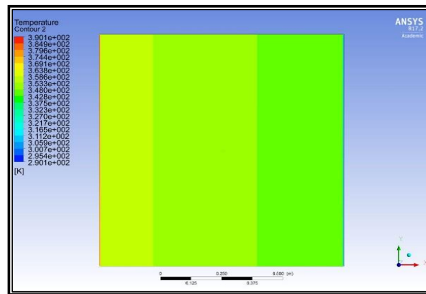
Fig 5b. Isotherms for silver-water nanofluid, Ra = 10^4 , no radiative flux with \Phi = 0.01 .
