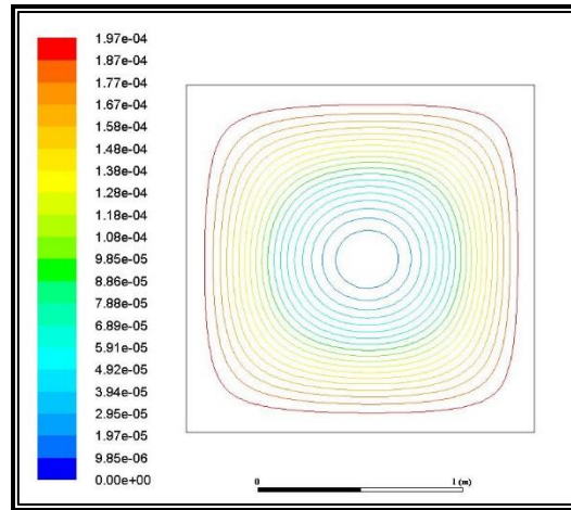
Fig 6a. Streamline distributions for silver-water nanofluid, Ra = 10^4 , P1 flux model with \Phi = 0.01 .
