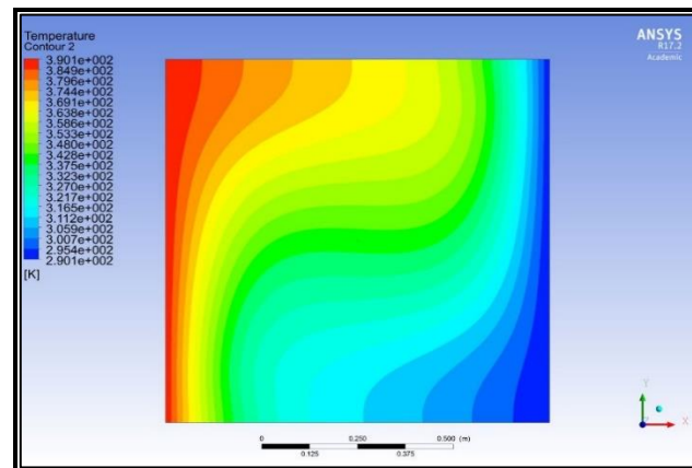
Fig 5c. Isotherms for silver-water nanofluid, Ra = 10^4 , P1 radiative flux with \Phi = 0.01 .
