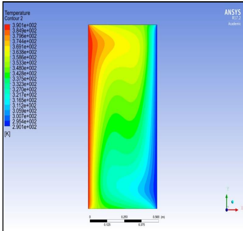
Fig 15. Isotherms for Titanium oxide-water nanofluid, PI flux with \Phi = 0.04 , Ra = 10^5 and absorption coefficient of 0.2 for aspect ratio AR = 2 .
