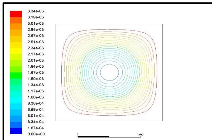
Fig 7d. Streamline distributions for silver-water nanofluid, Ra = 10^5 , no radiative flux with \Phi = 0.04 .
