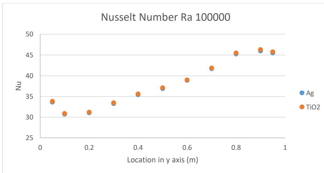
Fig 11. Nusselt numbers for different nanofluids, P1 flux with \Phi = 0.04 , Ra = 10^5 .
