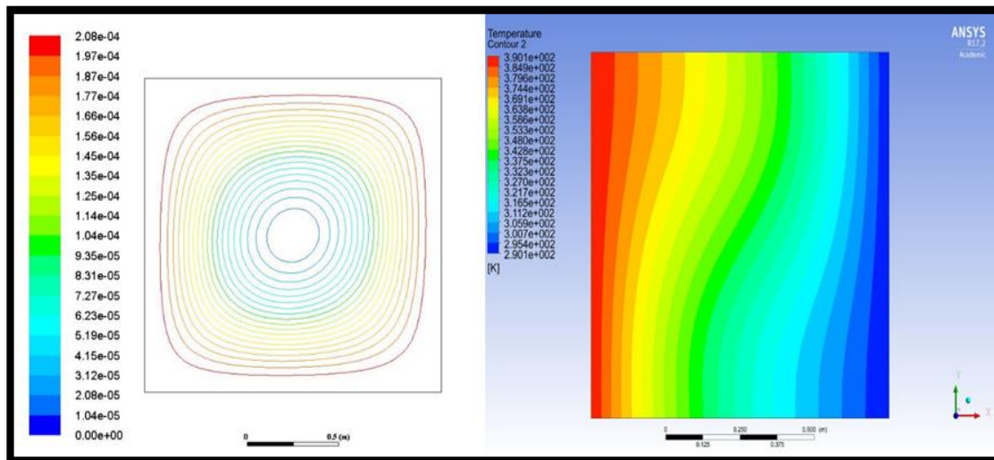
Fig A- finite volume results for Streamline and Isotherm plots for copper-water nanofluid, with a Rayleigh number of 10^3 , volume fraction of 0.01 (Abu-Nada, E., & Oztop, H. 2009)
