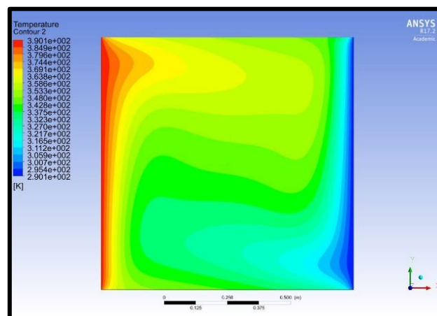
Fig 7a. Isotherms for silver-water nanofluid, Ra = 10^5 , P1 radiative flux with \Phi = 0.04 .
