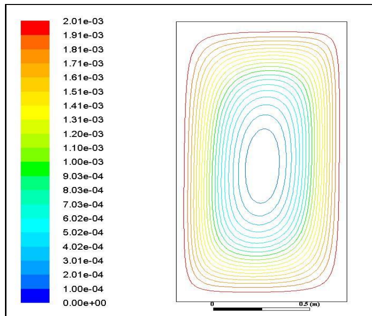
Fig 16. Streamlines for Titanium oxide-water nanofluid, PI flux with \Phi = 0.04 , Ra = 10^5 and absorption coefficient of 0.2 for aspect ratio AR = 2 .
