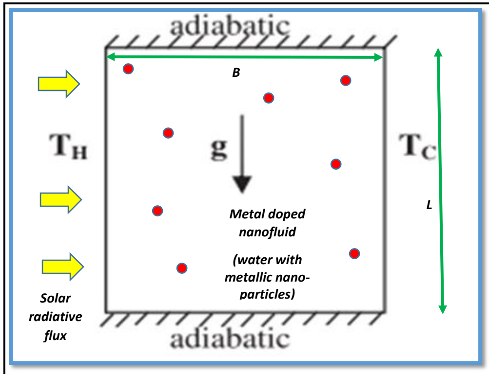
Fig. 1: Direct absorber solar nanofluid collector enclosure geometry
