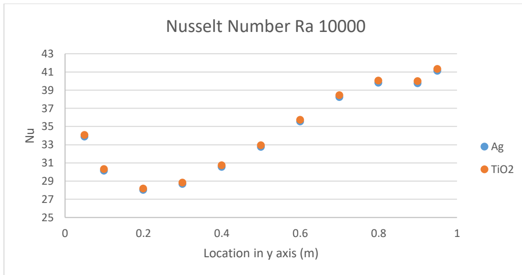
Fig 10. Nusselt numbers for different nanofluids, P1 flux with \Phi = 0.04 , Ra = 10^4 .
