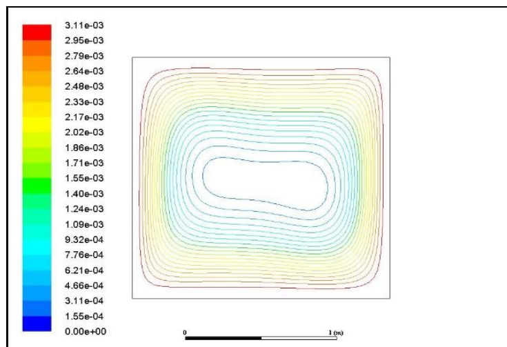
Fig 7c. Streamline distributions for silver-water nanofluid, Ra = 10^5 , P1 radiative flux with \Phi = 0.04 .
