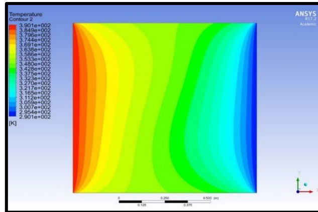
Fig 5a. Isotherms for silver-water nanofluid, Ra = 10^4 , Rosseland flux model with \Phi = 0.01 .
