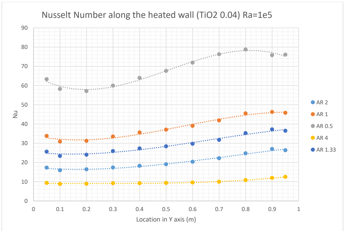
Fig 23. Nusselt numbers along hot wall for Titanium oxide-water nanofluid, P1 flux with \Phi = 0.04 , Ra = 10^5 with different enclosure aspect ratios (AR).
