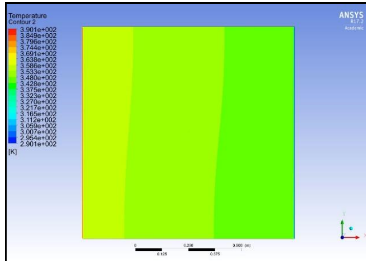
Fig 7b. Isotherms for silver-water nanofluid, Ra = 10^5 , no radiative flux with \Phi = 0.04 .
