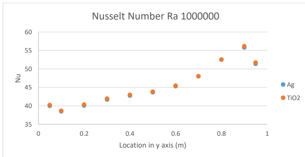
Fig 12. Nusselt numbers for different nanofluids, P1 flux with \Phi = 0.04 , Ra = 10^6 .
