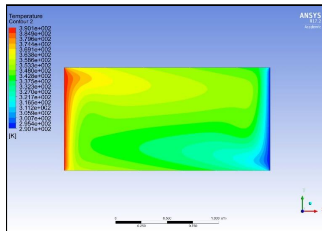
Fig 21. Isotherms for Titanium oxide-water nanofluid, PI flux with \Phi = 0.04 , Ra = 10^5 and absorption coefficient of 0.2 for aspect ratio AR = 0.5 (shallow cavity).
