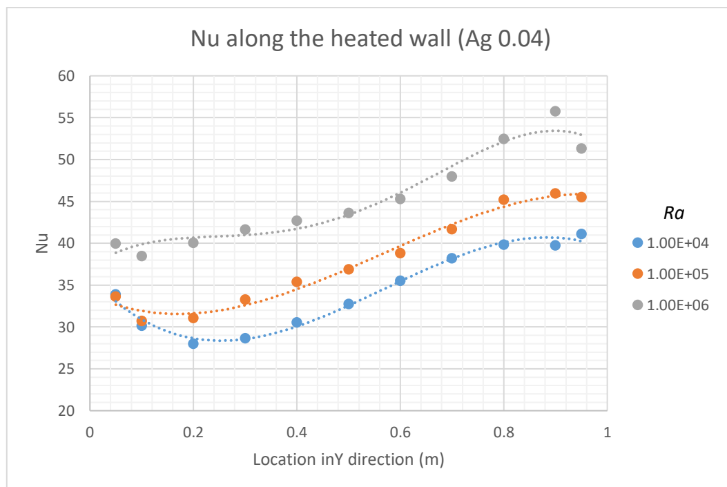
Fig 9. Nusselt numbers along hot wall for silver-water nanofluid, P1 flux with \Phi = 0.04 for different Rayleigh numbers.
