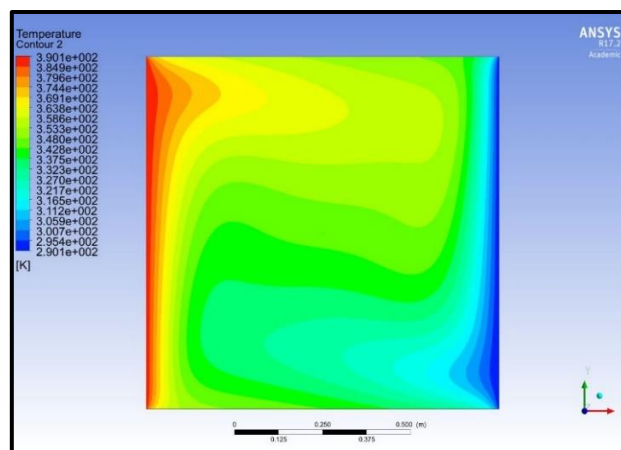
Fig 19. Isotherms for Titanium oxide-water nanofluid, PI flux with \Phi = 0.04 , Ra = 10^5 and absorption coefficient of 0.2 for aspect ratio AR = 1 (square cavity).
