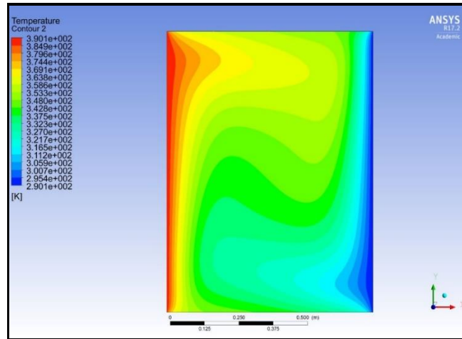
Fig 17. Isotherms for Titanium oxide-water nanofluid, PI flux with \Phi = 0.04 , Ra = 10^5 and absorption coefficient of 0.2 for aspect ratio AR = 4/3 .
