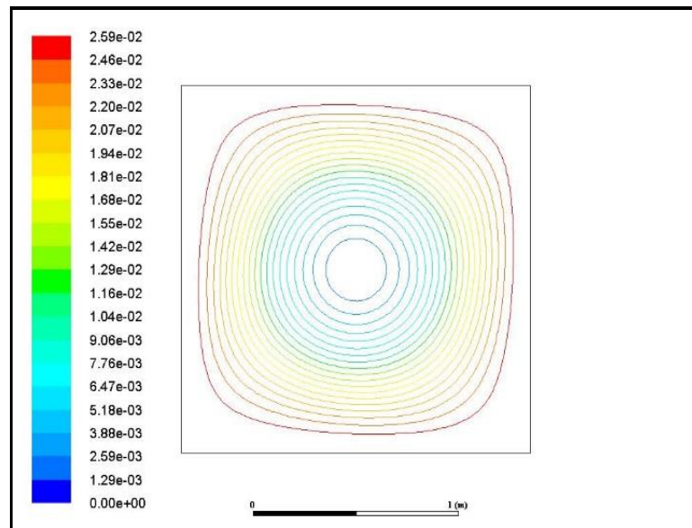
Fig 8d. Streamline distributions for silver-water nanofluid, Ra = 10^6 , no radiative flux with \Phi = 0.04 .
