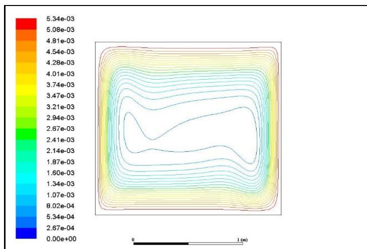
Fig 8c. Streamline distributions for silver-water nanofluid, Ra = 10^6 , P1 radiative flux with \Phi = 0.04 .
