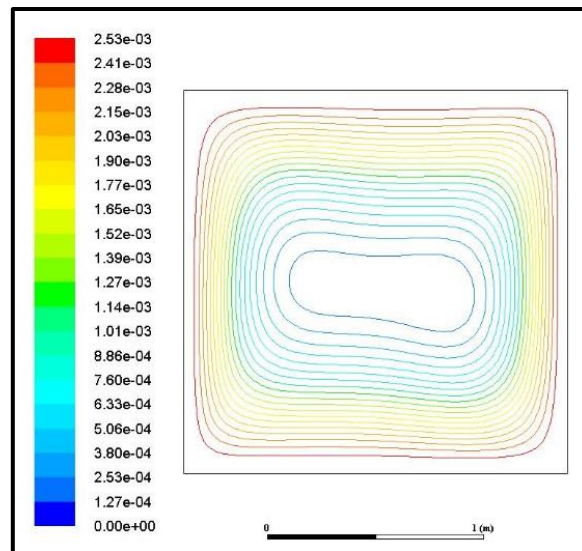
Fig 20. Streamlines for Titanium oxide-water nanofluid, PI flux with \Phi = 0.04 , Ra = 10^5 and absorption coefficient of 0.2 for aspect ratio AR = 1 (square cavity).
