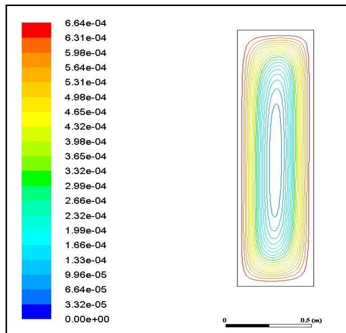
Fig 14. Streamlines for Titanium oxide-water nanofluid, PI flux with \Phi = 0.04 , Ra = 10^5 and absorption coefficient of 0.2 for aspect ratio AR = 4 .
