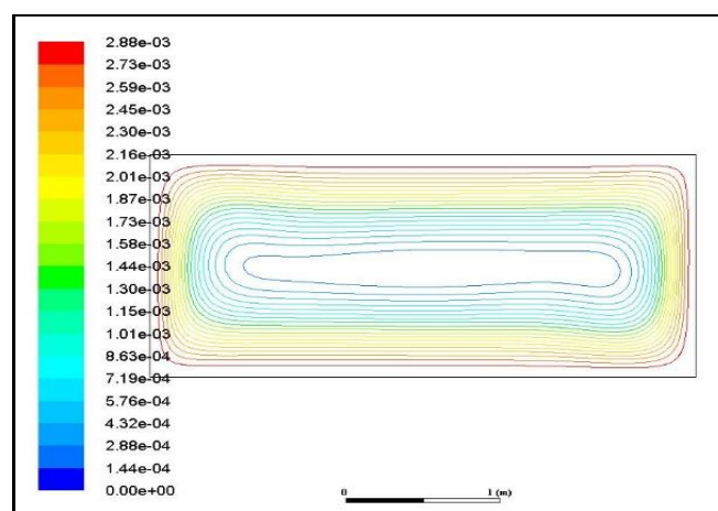
Fig 22. Streamlines for Titanium oxide-water nanofluid, PI flux with \Phi = 0.04 , Ra = 10^5 and absorption coefficient of 0.2 for aspect ratio AR = 0.5 (shallow cavity).
