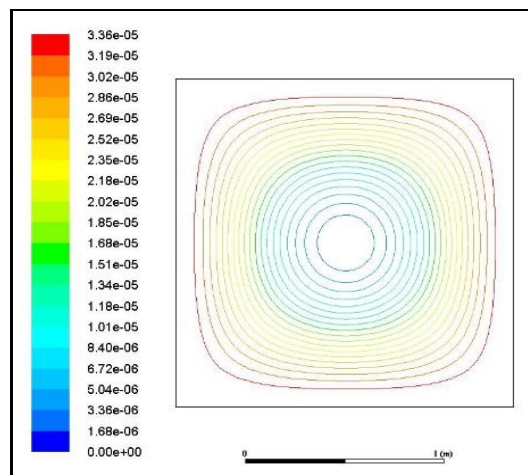
Fig 6b. Streamline distributions for silver-water nanofluid, Ra = 10^4 , Rosseland flux with \Phi = 0.01 .
