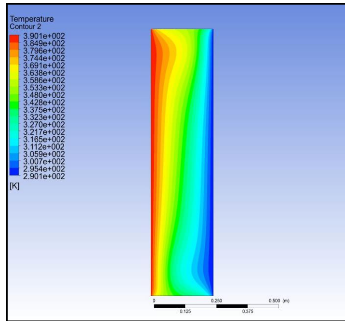
Fig 13. Isotherms for Titanium oxide-water nanofluid, PI flux with \Phi = 0.04 , Ra = 10^5 and absorption coefficient of 0.2 for aspect ratio AR = 4 (tall enclosure).
