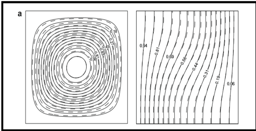
Fig A- finite volume results for Streamline and Isotherm plots for copper-water nanofluid, with a Rayleigh number of 10^3 , volume fraction of 0.01 (Abu-Nada, E., & Oztop, H. 2009)
