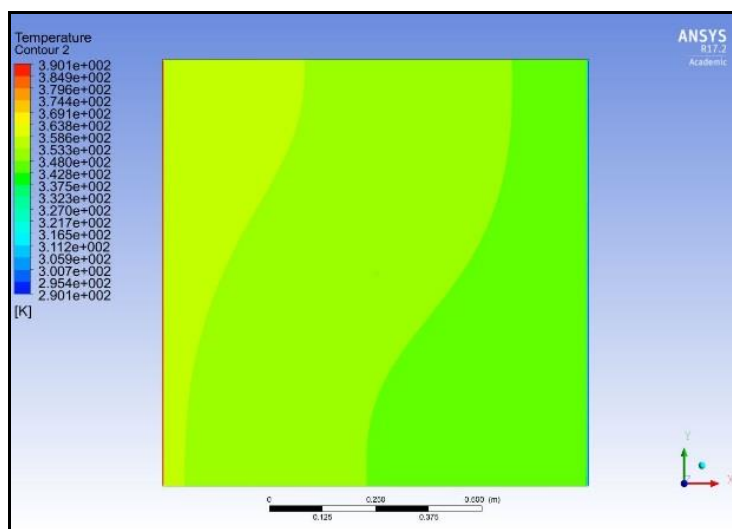
Fig 8b. Isotherms for silver-water nanofluid, Ra = 10^6 , no radiative flux with \Phi = 0.04 .
