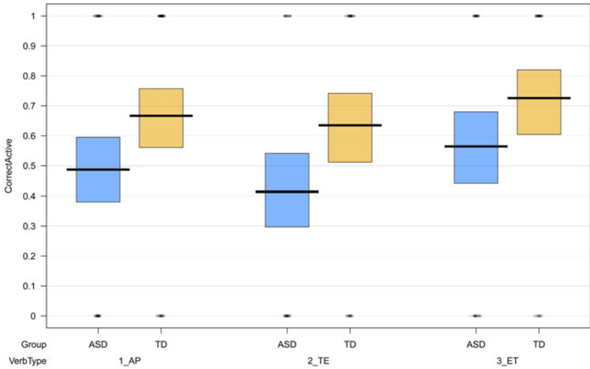
Figure 3. Correct Actives
