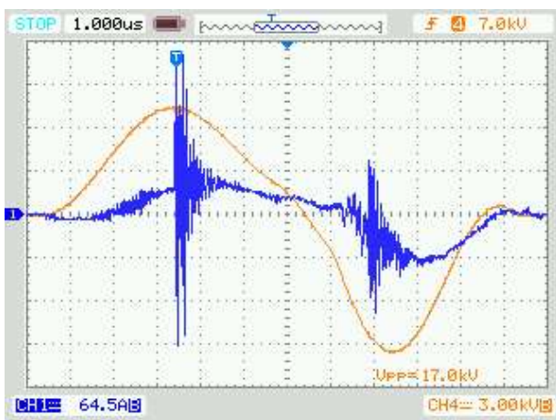
Fig. 2. Typical measured waveforms of pulsed voltage and current of the DBD reactor.
