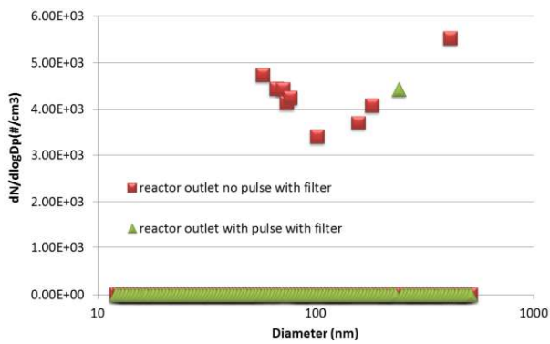
Fig. 7. Particle Size Distribution with filtering (2000rpm, 25% Load, 15kV pp and 10 KHz).
