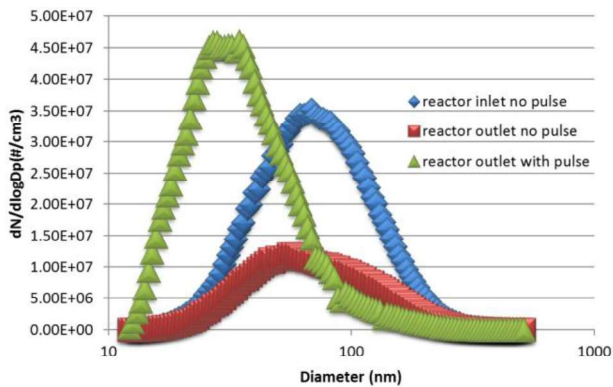
Fig. 4. Particle size distribution (2000rpm, 25% Load, 20kV pp and 10 kHz)
