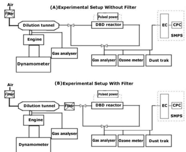
Fig. 3. Schematic diagram of experimental setup: (A) without filter-(B) with filter.
