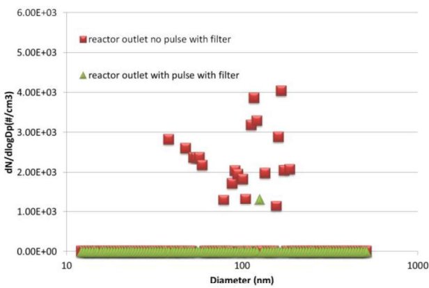
Fig. 8. Particle Size Distribution with filtering (2000rpm, 25% Load, 17kV pp and 10 KHz).
