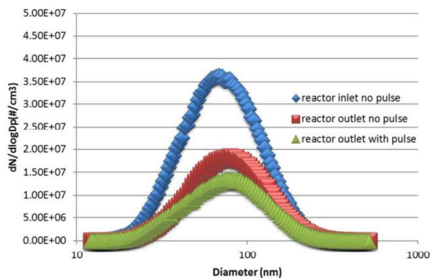
Fig. 5. Particle size distribution (2000rpm, 25% Load, 17kV pp and 10 kHz)
