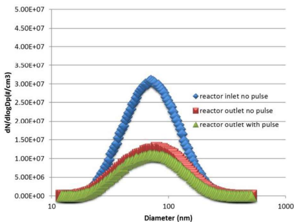
Fig. 6. Particle size distribution (2000rpm, 25% Load, 15kV pp and 10 kHz)
