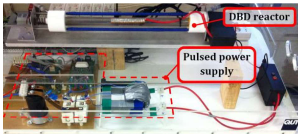
Fig. 1. Plasma reactor and electrical setup.
