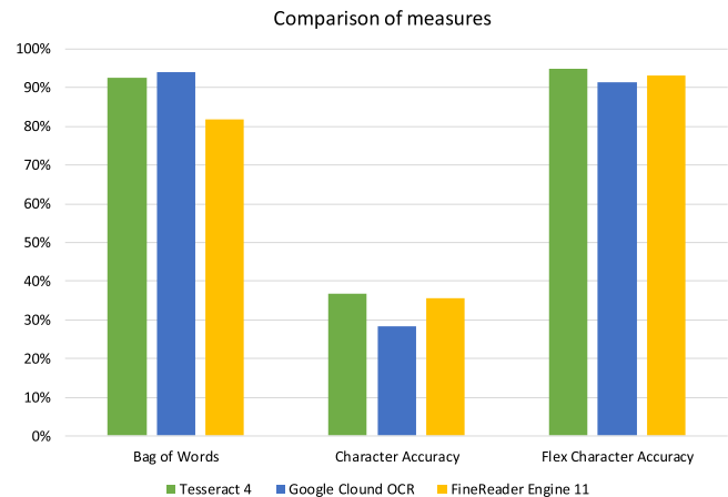
Fig. 6. Comparison of evaluation measures and OCR engines across all images in the example historical document dataset.
