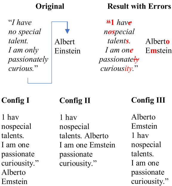
Fig. 3. Example with original text, result with errors, and different result text configurations. Character errors are indicated in red (substitutions in bold, deletions crossed out, insertions as plain red text).
