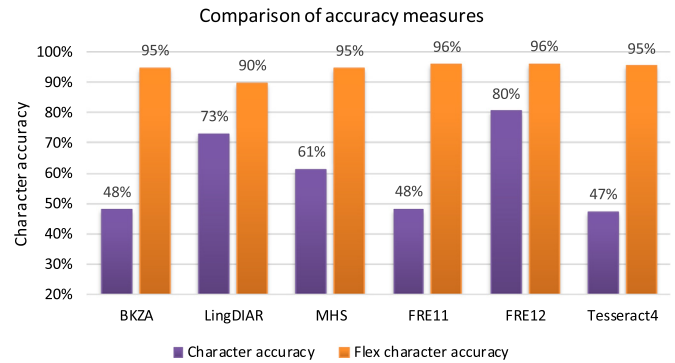
Fig. 8. Character accuracy and flex character accuracy for RDCL2019 submissions.
