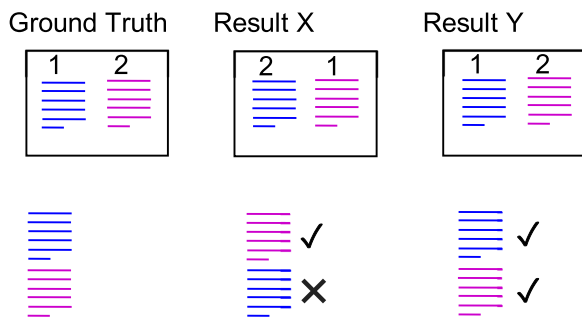
Fig. 1. Impact of reading order on Character Accuracy (top: paragraph order on page; bottom: serialised text). Given two paragraphs and the same system performance at the character level, the order in which the text is serialised is significant. OCR result X has the inverse paragraph order than the ground truth and will receive a low Character Accuracy score. OCR result Y has the same paragraph order as the ground truth and is likely to receive a higher Character Accuracy score.
