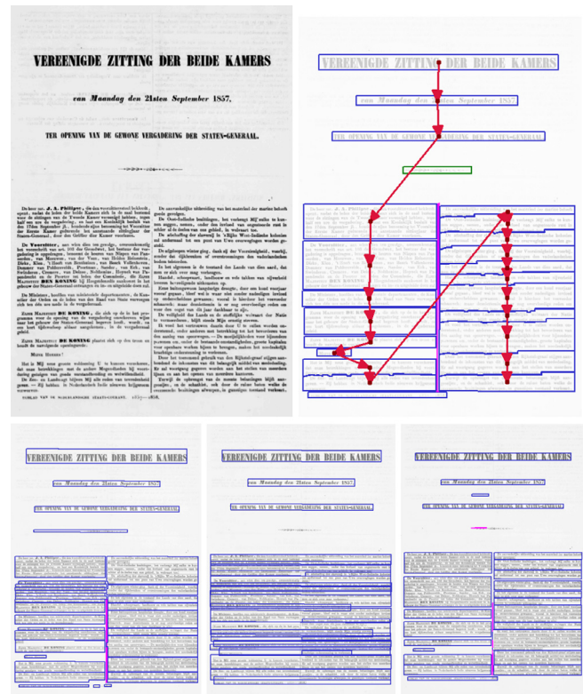
Fig. 5. First page of Dutch legal document from 1857 (“Handelingen der Staten-Generaal”), (top left: original image, top right: ground truth regions and reading order, bottom: OCR result regions - left: Tesseract 4, centre: Google OCR, right: FineReader Engine 11).
