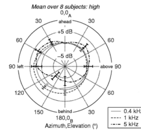
Figure 11: Directional loudness sensitivities at 65 dB SPL, reproduced from [22]
