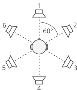
Figure 1: Loudspeaker set-up in the listening room.
