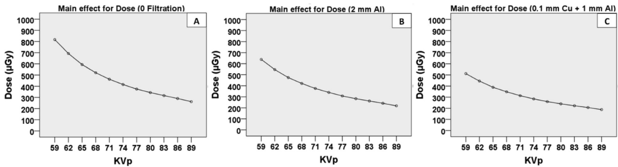
Fig. 4. (A, B and C): 10 year-old the main effect plots for dose ( \mu\text{Gy} ) when increasing the kVp; (A) at 0 filtration, (B) at 2 mm Al, (C) at 0.1 mm Cu + 1 mm Al.
