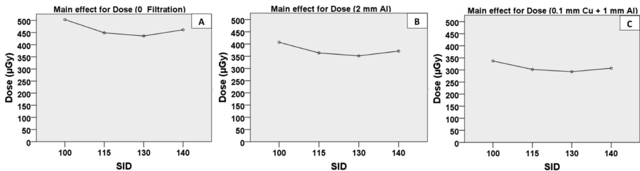
Fig. 6. (A, B and C): 10 year-old the main effect plots for dose ( \mu\text{Gy} ) when increasing the SID; (A) at 0 filtration, (B) at 2 mm Al, (C) at 0.1 mm Cu + 1 mm Al.
