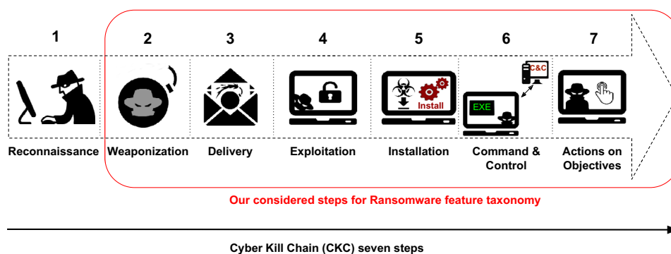
Fig. 2 Lockheed Martin Cyber Kill Chain (CKC) [22] seven steps. The part that is specified with the red rectangle highlights six steps that we considered in our ransomware feature taxonomy
