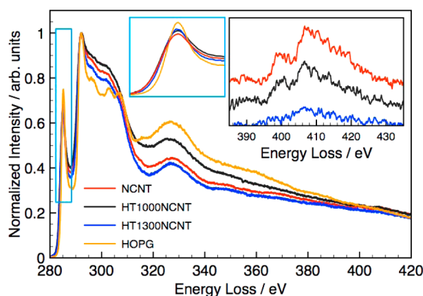
Figure 2. Magic-angle 55 C 1s core excitation EELS spectra for NCNT (red curve); HT1000NCNT (black curve); HT1300NCNT (blue curve) and HOPG (orange); Insets: N 1s EELS spectra (black inset) and detail of the \pi^* resonance (blue-border inset).
