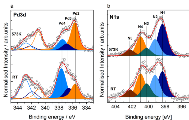
Figure 11. Core level spectra at 600 eV KE for the sample PdCl 2 NCNT during in situ reduction (a) Pd 3d and (b) N 1s.
