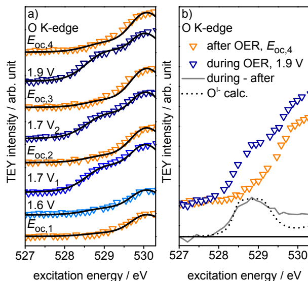
Fig. 3 a) Low excitation energy region of O K-edges of Ir-coated PEM (60 s Ir sputtered), consecutively recorded (bottom to top) in the three-electrode cell with the indicated potentials vs. SHE applied and b) difference spectrum of two consecutively recorded O K-edges and comparison with calculated \text{O}^{\text{I-}} spectrum (ring current=13 mA, p=0.45 Pa, 0.1 M \text{H}_2\text{SO}_4 ).
