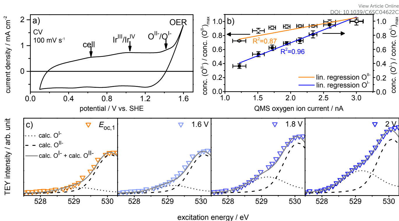
Fig. 2 a) Cyclic voltammogram, b) normalized \text{O}^{\text{II-}} and \text{O}^{\text{I-}} concentrations over QMS oxygen ion current, and c) zoomed and fitted low excitation energy regions of O K-edges recorded in the three-electrode cell (indicated potentials vs. SHE, ring current=60 mA, p=0.3 Pa, 0.1 M \text{H}_2\text{SO}_4 ).
