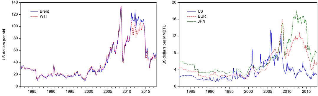
Figure 1. Plots of Crude oil and natural gas prices
