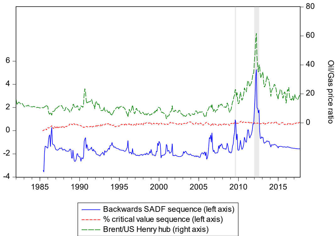
Figure 7. Multiple bubbles in the US oil-gas ratio
