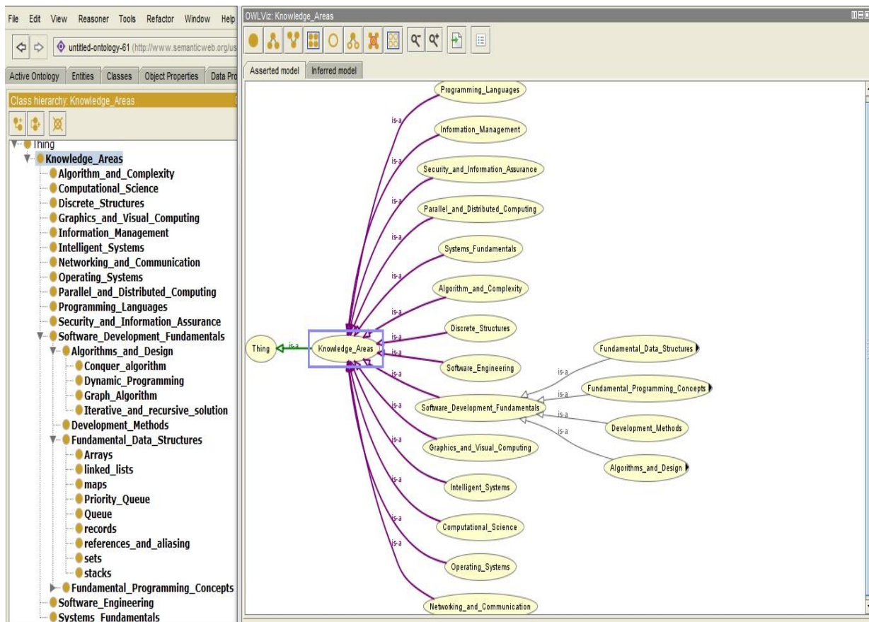
Fig. 2. A screenshot of the computer science ontology
