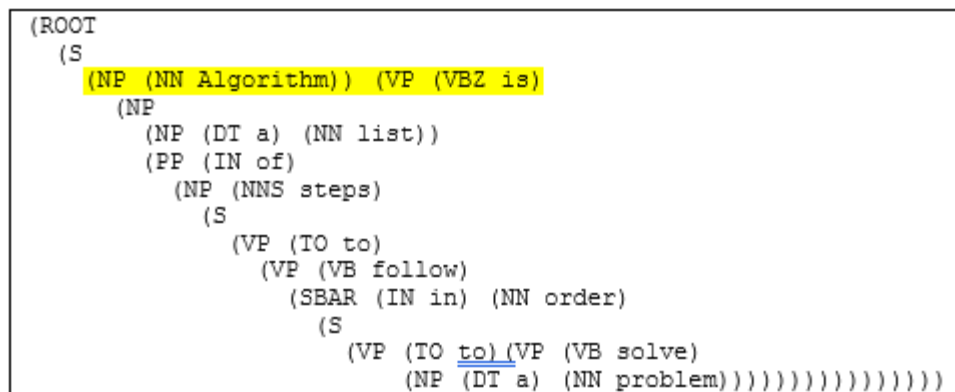
Fig. 6. A sample parse tree using the Stanford Parser
