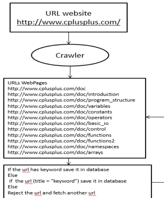
Fig. 4 Crawler process in the APELS system
