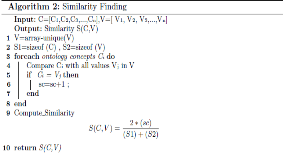
Fig. 3: The similarity measure algorithm
