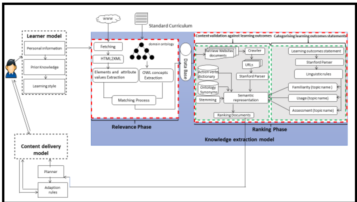
Fig. 1 System architecture showing the different models of the APELS system
