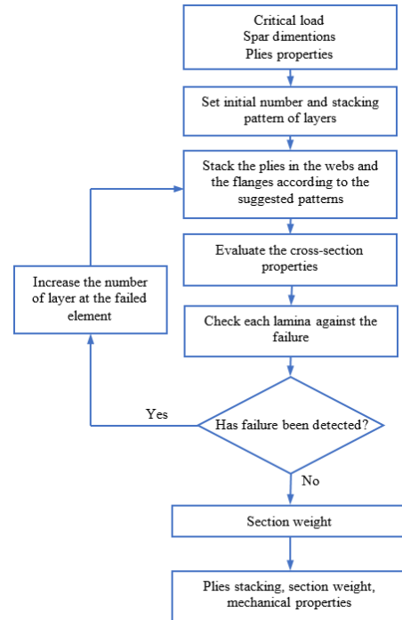
Figure 4. Cross-section design methodology
