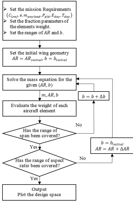
Figure 1. Conceptual design approach to explore the design space
