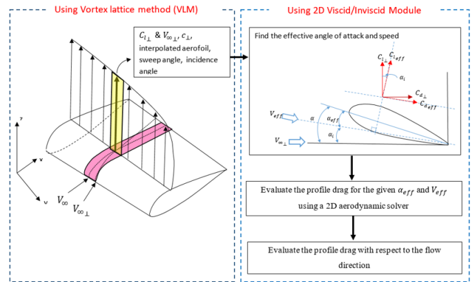
Figure 3. Procedure of the Quasi 3D Aerodynamic model
