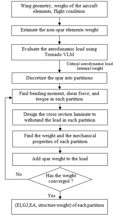
Figure 2. Overview of the wing sizing methodology
