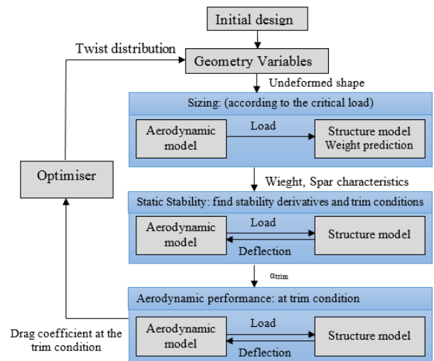
Figure 5. Optimisation Architecture
