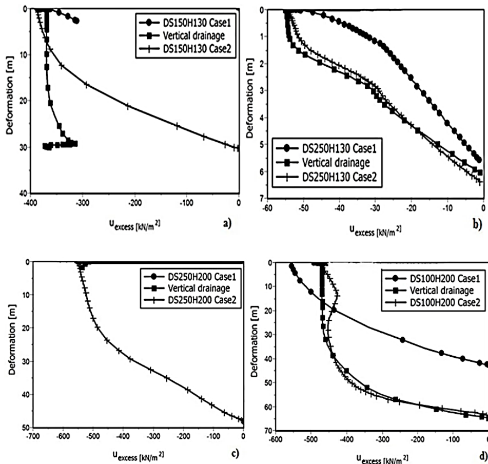
Figure 2: Effect of different drainage scenarios under the calculated coefficient of permeability ( k_c^2 ) at 55kPa (Where: case 1 is the horizontal drainage scenario and case 2 is combined vertical and horizontal drainage)
