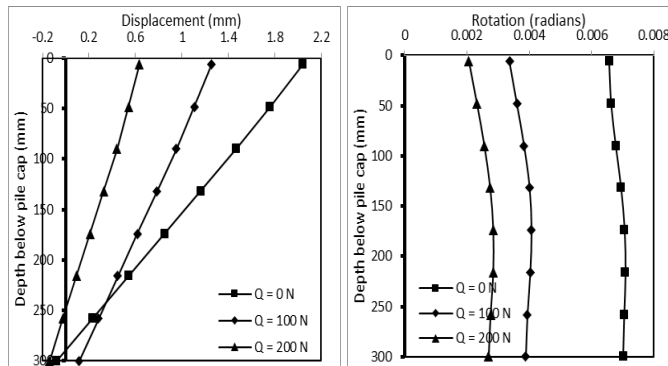
a. Deflection of the front pile b. Rotation of the front pile Fig. 11 Rotation and deflection profiles at different levels of axial load.
