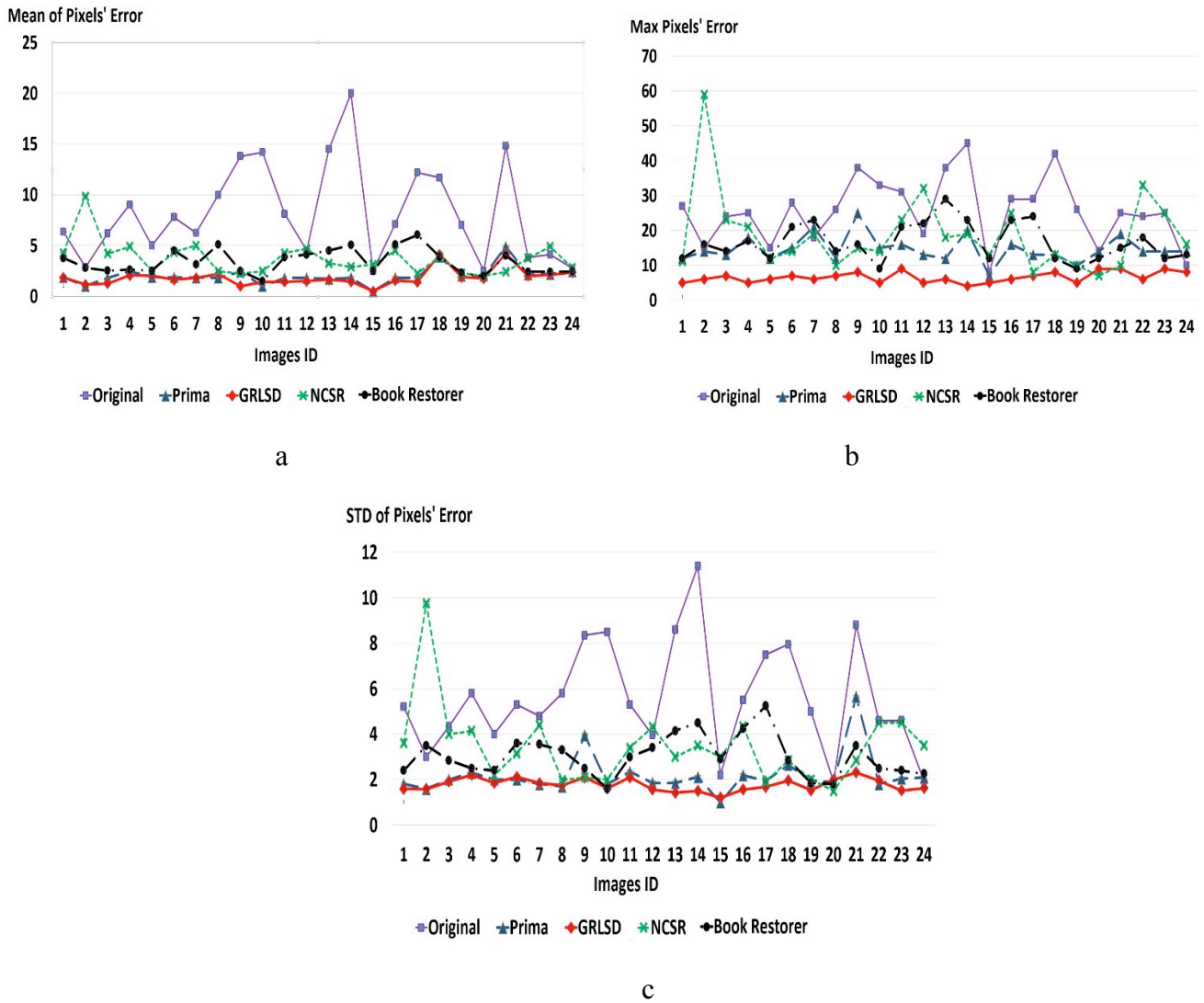
Fig. 13. Evaluation results of NCSR, Book Restorer™ and proposed method on SME, MPE, SDE. a) Evaluation results on Mean of Pixel's Error. b) Evaluation results on Max of Pixels' Error. c) Evaluation results on STD.
