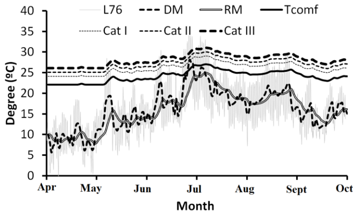
Figure 3 The limiting comfort temperature for the year of 1976 using Eq. 03 for April to September (the upper limits of Category I, II & III would be a parallel shift of T_{comf} by 2, 3 & 4 degree Celsius).
