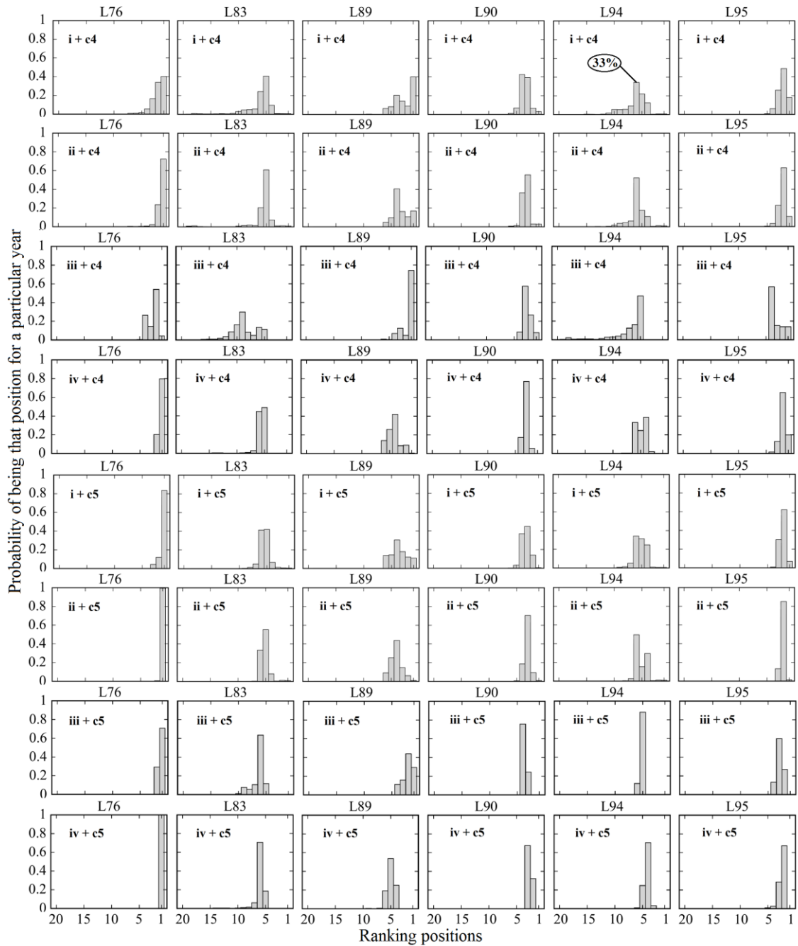
Figure 9 [samples i to iv + c4, c5] Ranking probabilities by both ‘the number of hours over’ and ‘adh over’ BS EN 15251 Category II upper limit ( ref : Table 5) for the single zone office space during occupancy.
