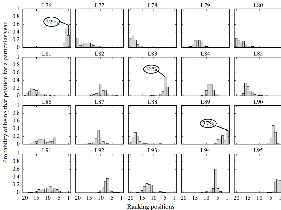
Figure 4 [sample i + c0] – Ranking probability by the number of hours over 28°C for the single zone office space during occupancy.
