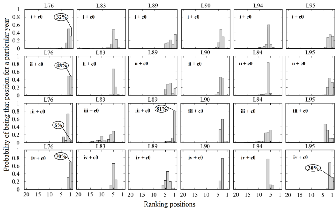
Figure 6 [samples i to iv + c0] Ranking probabilities by the ‘number of hours over’ 28°C (ref: Table 5) for the single zone office space during occupancy.
