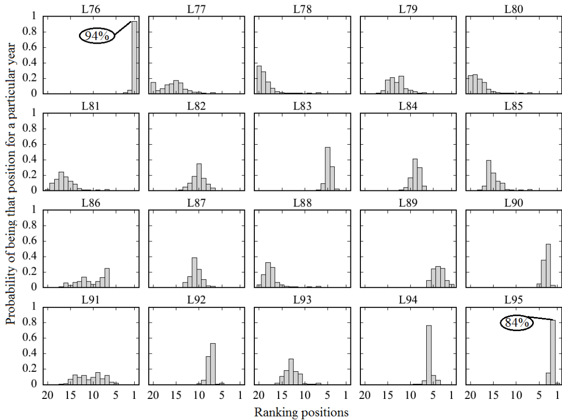
41 Figure 5 [sample i + c1] – Ranking probability by the number of accumulated degree 42 hours over 28°C for the single zone office space during occupancy. 43 44
