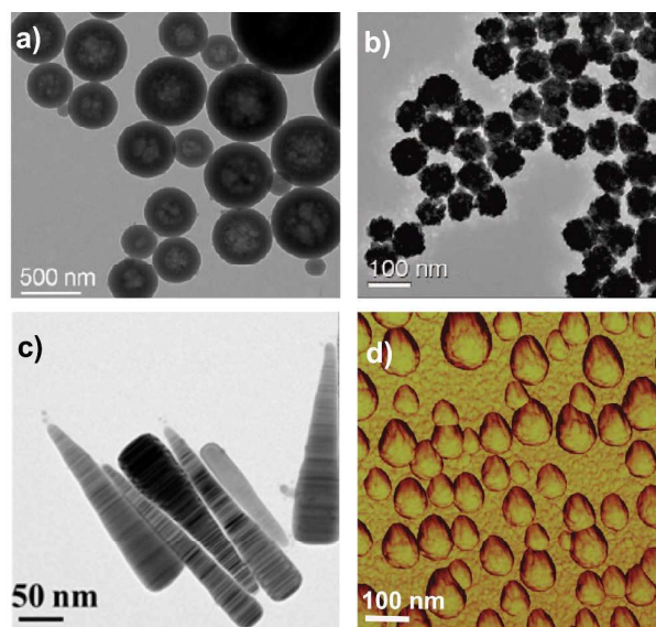
Figure 2: Examples of exotic shape of NPs in the literature: a) polymeric nanodisco balls (TEM micrograph) 36 , b) gold nanoflowers (TEM micrograph) 42 , c) silver nanocarrots (TEM micrograph) 45 , d) polymeric nanoraspberries (phase AFM image) 46 . Reprinted with permission from American Chemical Society.
