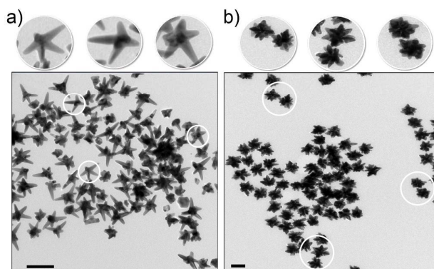
Figure 5: TEM micrographs of so-called, a) gold nanostars and b) gold short-tipped nanostars (also referred to as urchin-like nanoparticles). The insets underline the remarkable shape variation between the objects in the sample despite the classification as stars. Scale bars are 100 nm.
