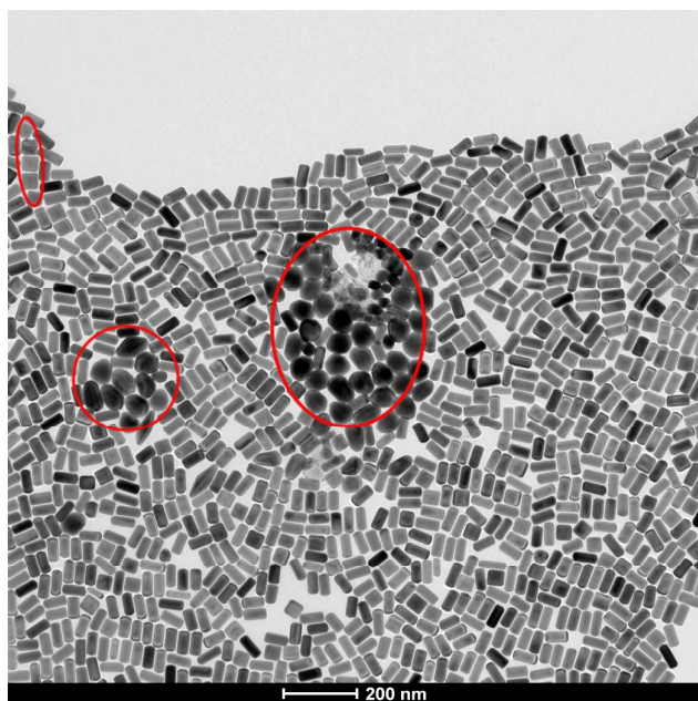
Figure 4: TEM micrograph of “exceptionally” shaped nanoparticles (red circles) in the same batch of seemingly monodisperse gold nanorods.
