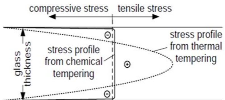
Figure 7. Residual stresses in toughened glasses [14]
