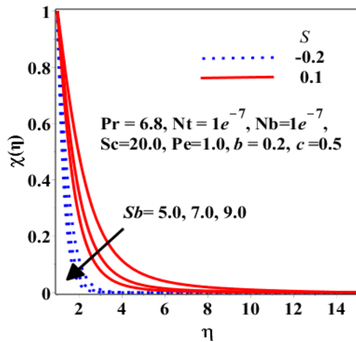
Figure 4: Effect of unsteadiness ( S ) and bioconvection Schmidt number ( Sb ) on the dimensionless motile microorganism density function.
