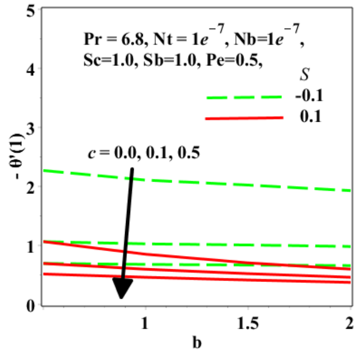
Figure 5: Effect of velocity slip ( b ) and thermal slip ( c ) parameters on the wall heat transfer rate.
