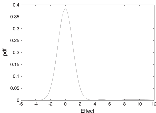
Figure 1. The four-parameter mixed skew distribution with u = 1, \mu = 0, \alpha = 0.5 and r = 10 . Note the bimodality
