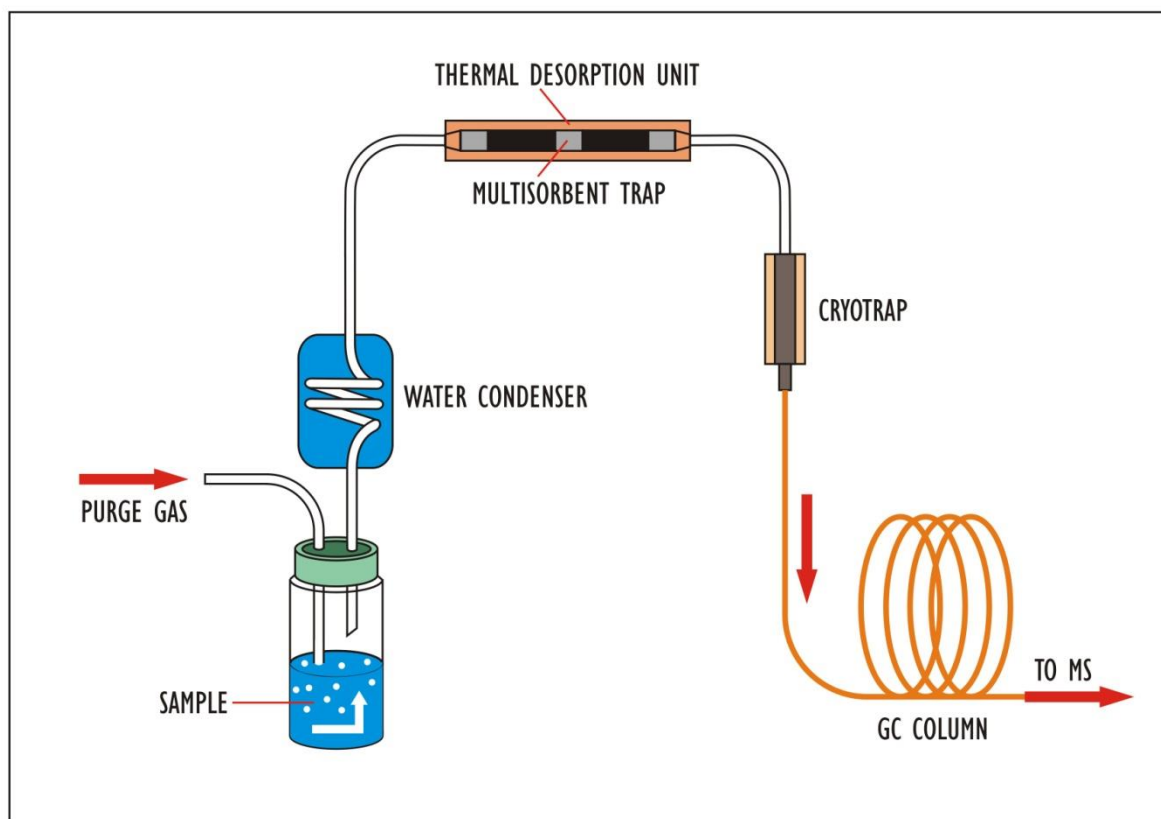
Figure 1: Diagram of analysis with on-line purge and trap-gas chromatography-mass spectrometry (PT-GC-MS).
