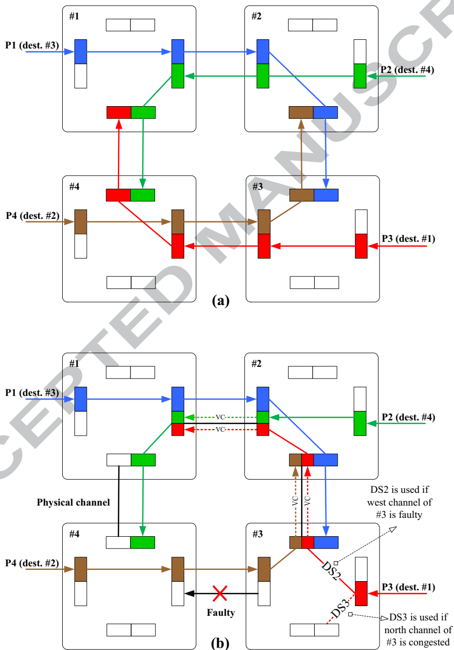
Fig. 7. A 4x4 NoC system: (a) fault-free system and (b) one link is faulty
