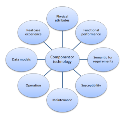
Figure 3- Database schema
