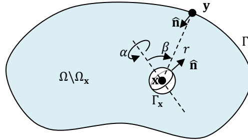
Figure 1: Geometry showing how the singularity at x is removed from the domain \Omega .
