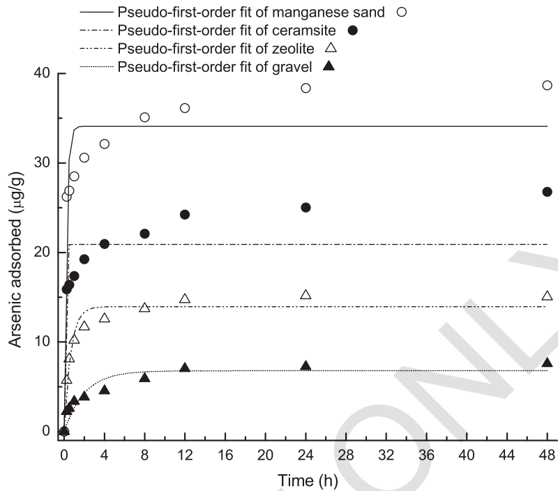
Figure 1. Pseudo-first-order kinetic model fitted for arsenic(V) adsorption to gravel, zeolite, ceramsite and manganese sand as a function of time.
