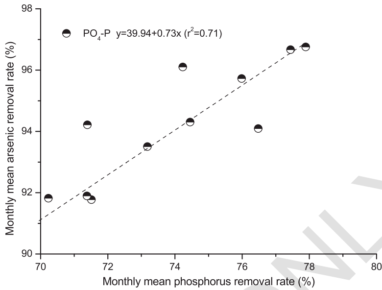
Figure 5. Higher monthly mean arsenic(V) removal rates observed at higher ortho-phosphate-phosphorus (PO 4 -P) removal rates for the selected representative wetland D.
