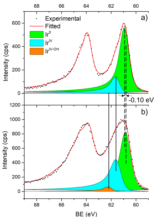
Fig. 7 High resolution Ir 4f spectra of fresh samples, (a) Ir/graphite and (b) Ir/GCN. For clarity, the comparison of the fitted contributions is limited to the \text{Ir}^0_{7/2} components without any satellite.
