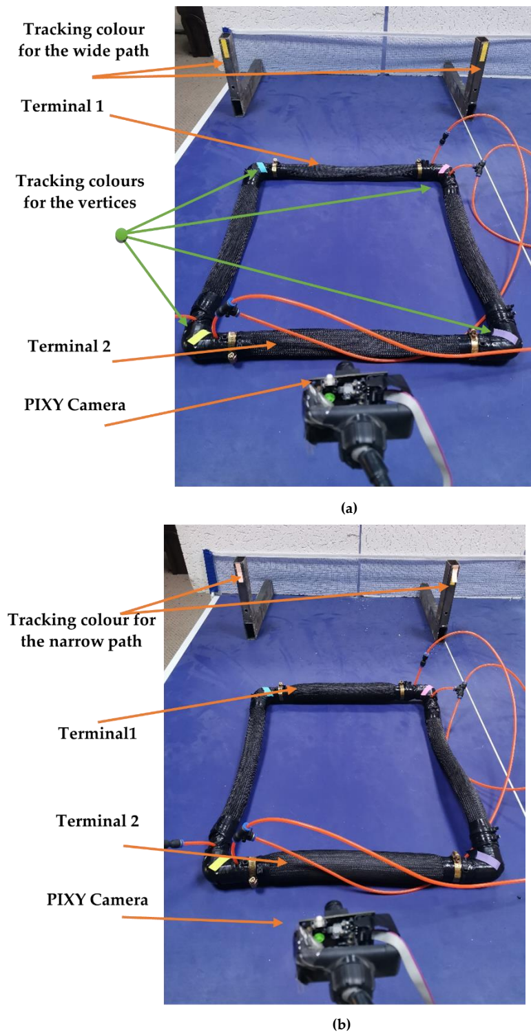
Figure 10. The shape change process. (a) A4SMR is the wide path. (b) A4SMR is the narrow path.
