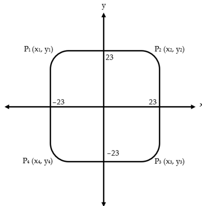
Figure 14. The mobile robot shape at rest condition.
