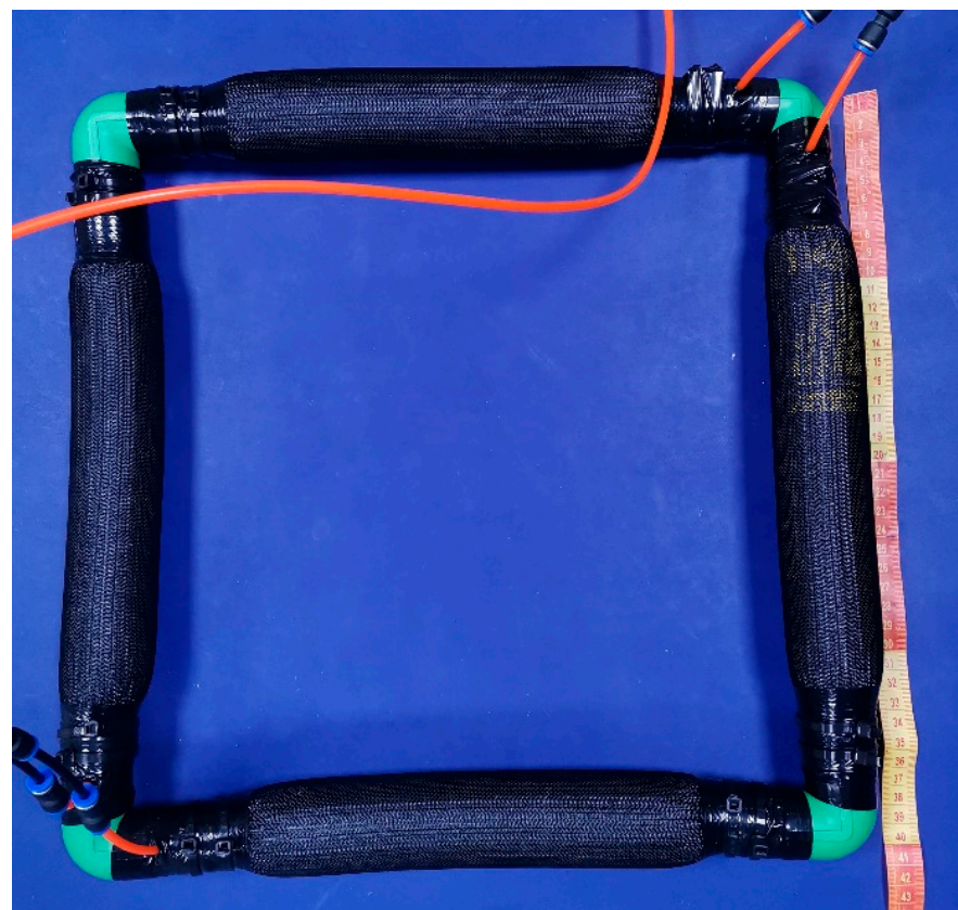
Figure 12. The proposed shape-shift mobile robot at 200 kPa.
