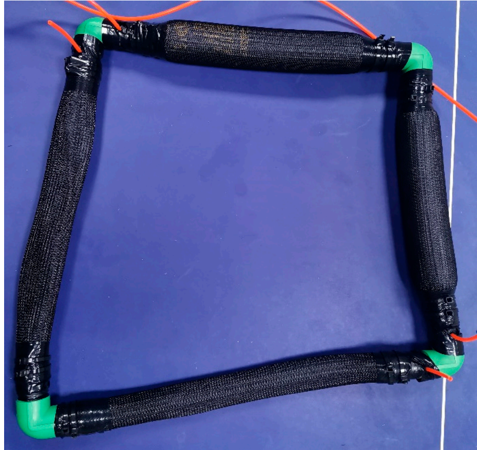
Figure 13. Irregular quadrable robot form.
