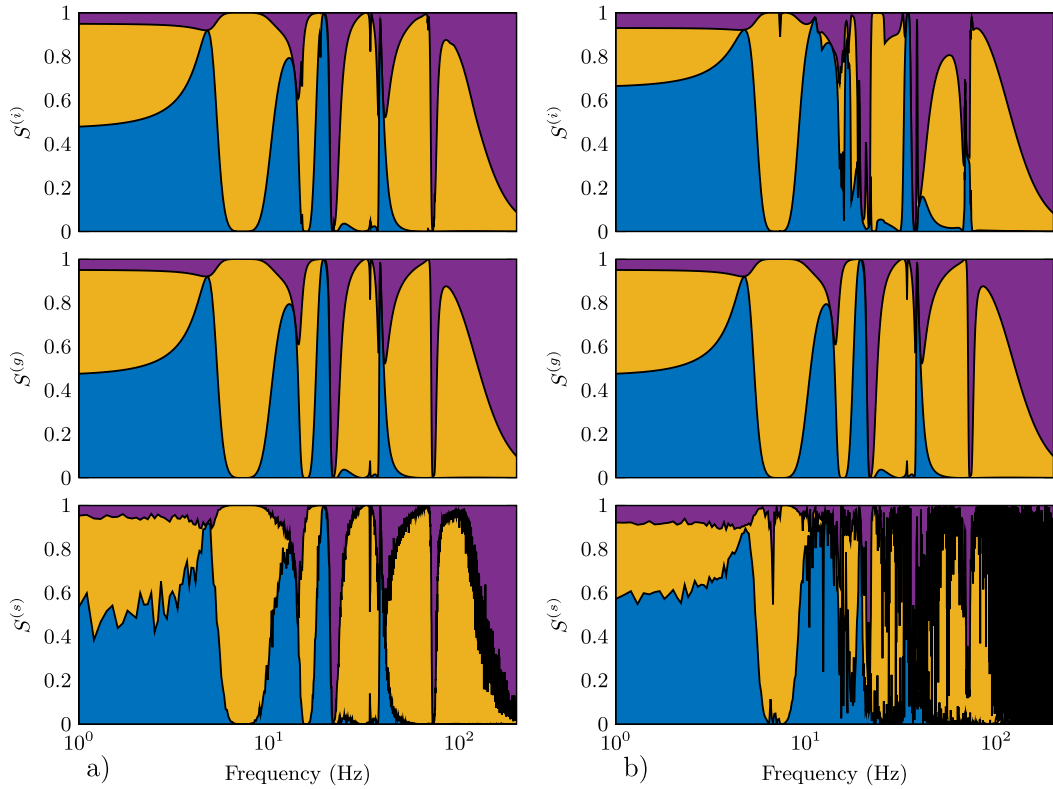
Fig. 9. Comparison of the interval (top), gradient (middle), and sample-based (bottom) sensitivity metrics for the minimum stiffness bounds Z_n = 1 \times 10^8(1+i) (a) and Z_n = 100(1+i) (b): S_1^{(i)} - blue, S_2^{(i)} - yellow, S_3^{(i)} - purple. (For interpretation of the references to colour in this figure legend, the reader is referred to the web version of this article.)
