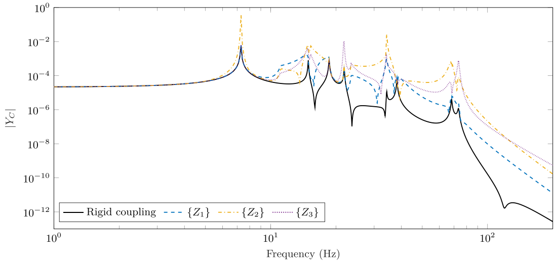
Fig. 7. Comparison of the upper bound on |Y_{1,1}| due the relaxation of each interface joint such that \{Z_n\} = [100 \ \infty] + i[100 \ \infty] . Rigid coupling is shown in black. Lower bounds are omitted for clarity.
