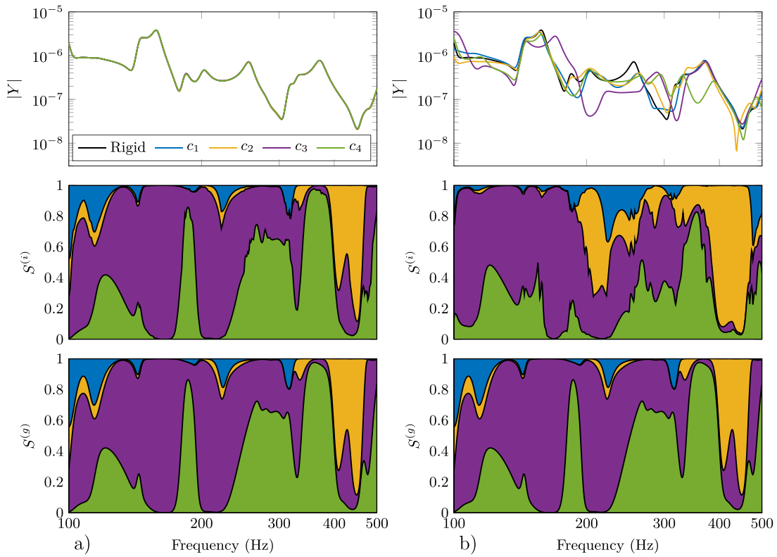
Fig. 12. Comparison of the interval (middle) and gradient (bottom) based sensitivity metrics for minimum stiffness bounds \underline{Z}_m = 1 \times 10^8(1 + i) (a) and \underline{Z}_m = 1 \times 10^5(1 + i) (b). Each metric describes the sensitivity of the transfer admittance with respect to a specific connection point, including both its translational and rotational DoFs: S_1^{(\square)} - blue, S_2^{(\square)} - yellow, S_3^{(\square)} - purple, S_4^{(\square)} - green. Shown in the top figures are the transfer admittances obtained by independently relaxing the DoFs at each connection point by an amount equal to the minimal stiffness bound. In black is the response obtained from the rigid assembly. (For interpretation of the references to colour in this figure legend, the reader is referred to the web version of this article.)
