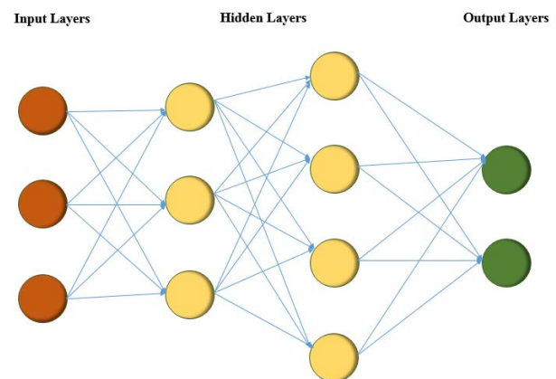
FIGURE 8. Neural network.
