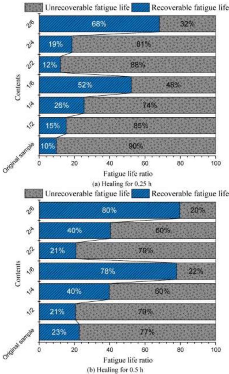
Figure 14. Fatigue life ratio of asphalt binder [62].
