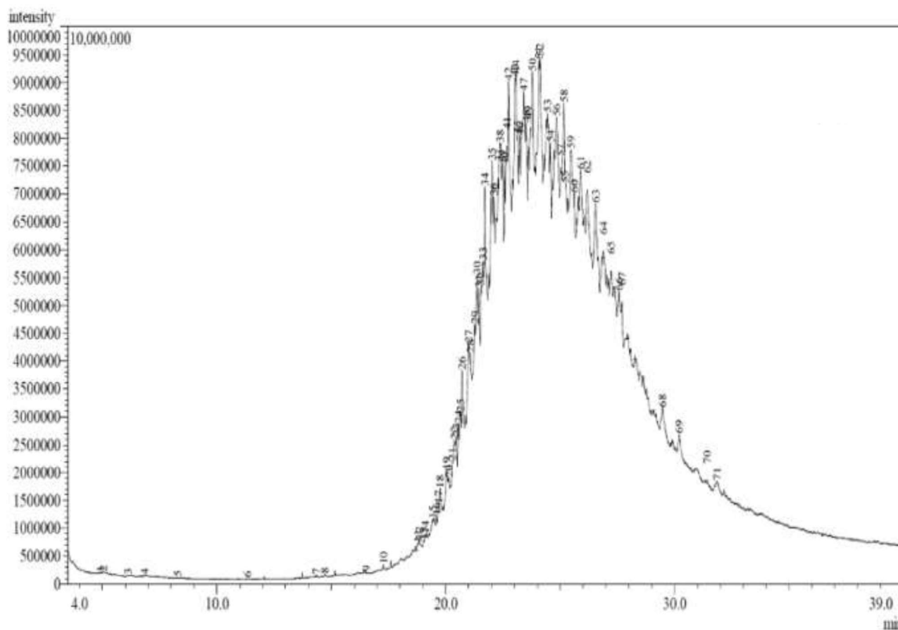
Figure 2. GC-MS results of WEO [15].
