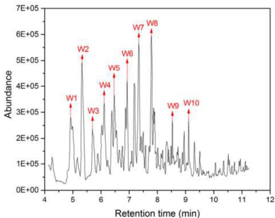
Figure 3. GC/MS chromatogram of WEO [18].
