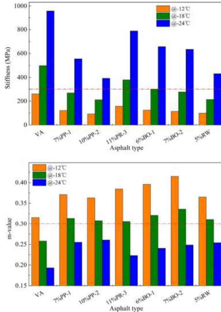
Figure 8. The behaviour of asphalt at low temperatures in terms of stiffness and m-value [71].
