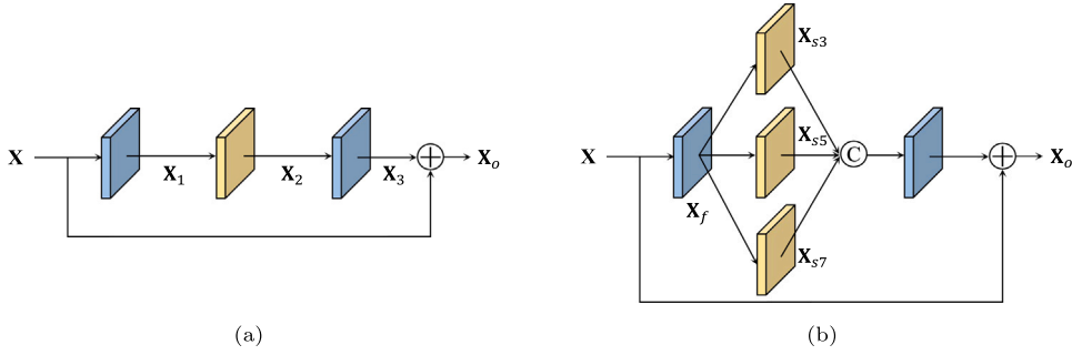
Fig. 2. The structure of the different linear bottleneck modules. (a) means the common linear bottleneck module; (b) denotes the proposed high-level linear bottleneck module (HLLB). The sub-modules marked in yellow and blue are the depthwise convolution and the standard convolution. \oplus stands for an elementwise addition layer.
