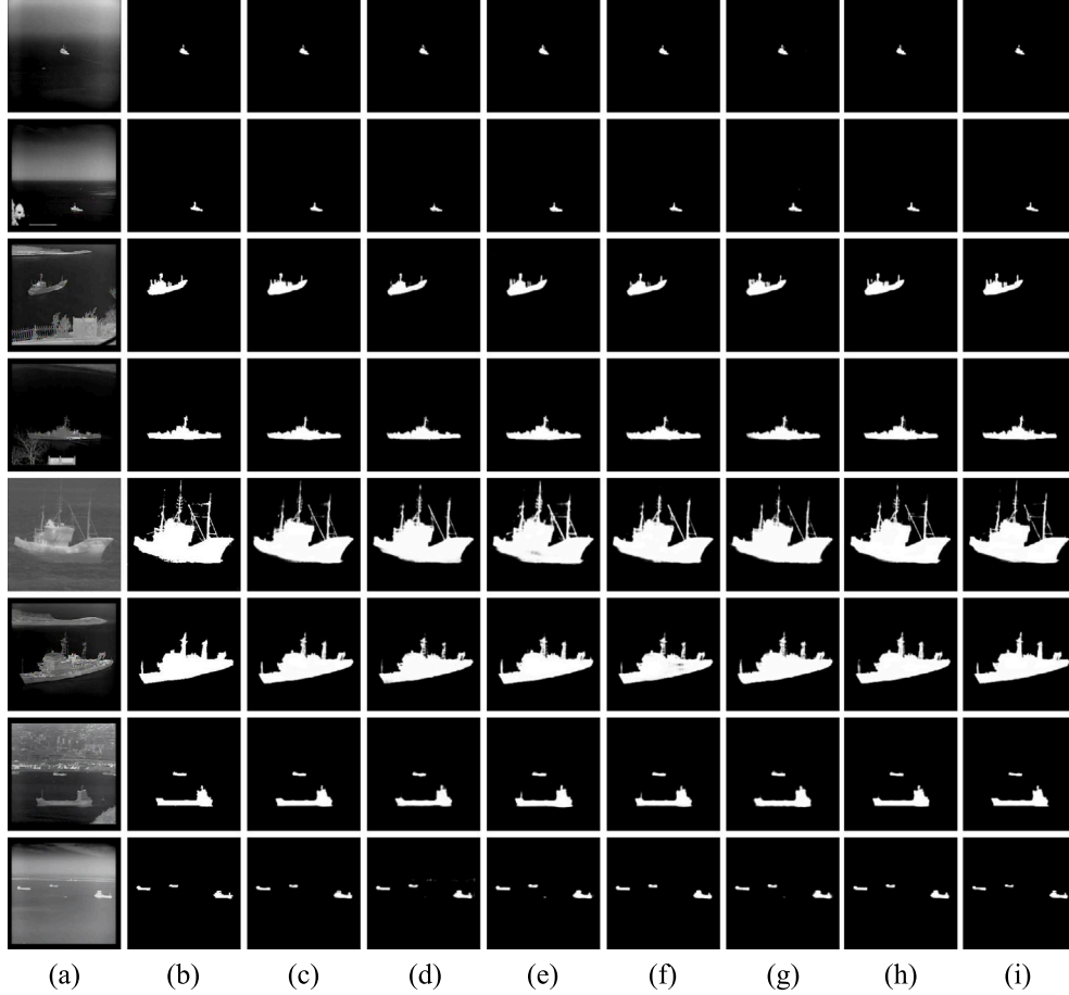
Fig. 7. Qualitative results comparison of ablation study. (a) input image. (b) groundtruth. (c) w/o AvgPool. (d) w/o Edge. (e) w/o DMIM. (f) w/o HLLB. (g) w/o MCIM. (h) w/o SAMM. (i) TBENet.
