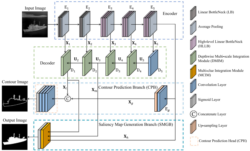
Fig. 1. The entire structure of TBENet. Our model is composed of four parts: an encoder, a decoder, a contour prediction branch, and a saliency map generation branch. The encoder-decoder network progressively produces fine-grained features. Given the refined features, the contour prediction branch delineates clear target contour. Guided by the contour information, the saliency map generation branch aggregates multi-dimensional information to obtain high quality saliency map.
