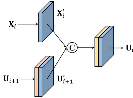
Fig. 3. The details of the depthwise multi-scale integration module (DMIM). The sub-module marked in pink stands for a up-sampling layer.
