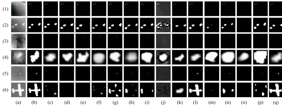
Fig. 11. Qualitative results of various methods on the IRSTD-1k dataset. (a) input image. (b) groundtruth. (c) NLDF. (d) PoolNet. (e) BASNet. (f) EGNet. (g) ITSD. (h) GCPANet. (i) F 3 Net. (j) BPFINet. (k) TSERNet. (l) DG-Light-NLDF. (m) RCSBNet. (n) R 2 Net. (o) DSLDRNet. (p) A3Net. (q) Ours. The targets are denoted by a green bounding box in the first, third, and fifth rows. And the second, fourth, and sixth rows present the magnified objects.
