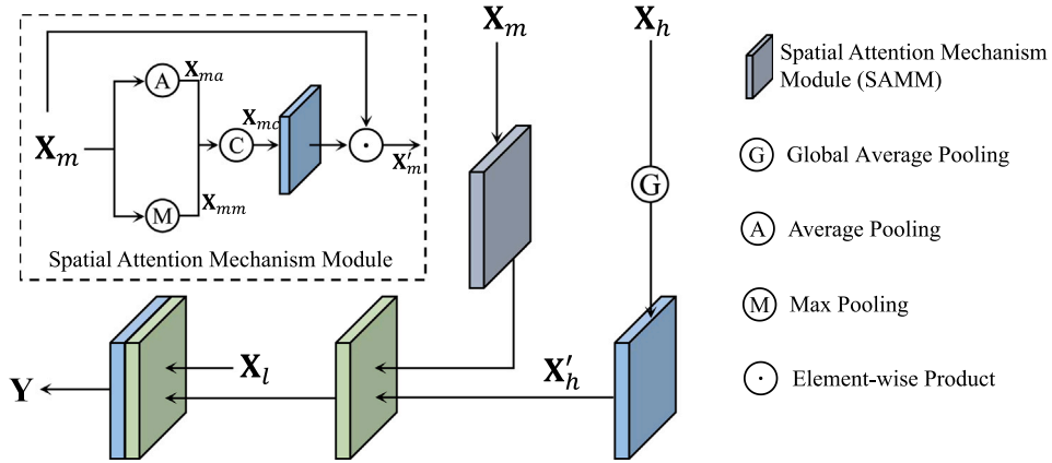
Fig. 4. The structure of the multi-cue integration module (MCIM). The input to the network consists of three parts, i.e., high-level semantic information X_h , mid-level spatial information X_m , and low-level detail information X_l . The MCIM first fuses mid-level features and high-level features, and the result is then fused with low-level features. By integrating information from multiple dimensions of the target, MCIM is able to produce informative features that enhance the detection performance of the model.
