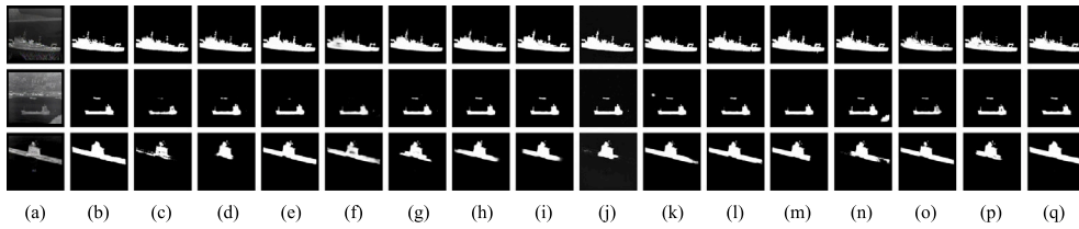
Fig. 6. Prediction results of various methods on the Small-IRShip dataset. (a) input image. (b) groundtruth. (c) NLDF. (d) PoolNet. (e) BASNet. (f) EGNet. (g) ITSD. (h) GCPANet. (i) F 3 Net. (j) BPFINet. (k) TSERNet. (l) DG-Light-NLDF. (m) RCSBNet. (n) R 2 Net. (o) DSLRDNet. (p) A3Net. (q) Ours.
