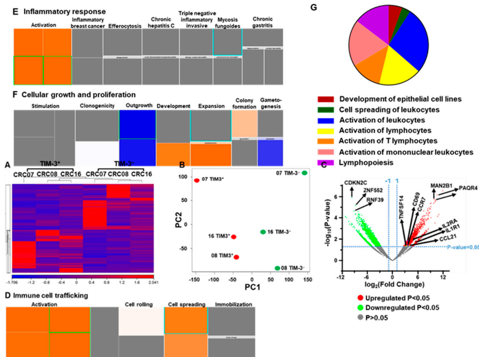
Figure 3. Differential gene expression of CD4^+TIM-3^+ and CD4^+TIM-3^- TILs. Hierarchical clustering of three TIM-3^+ and three TIM-3^- libraries (from patients CRC07, 08, and 16) on differentially expressed RNA transcripts from RNA-Sequencing data. Each column represents a sample and each row represents a transcript. Expression level of each gene in a single sample is depicted according to color scale (A). PCA plot shows the clustering of RNA transcriptome from of three TIM-3^+ and TIM-3^- libraries (B). Volcano plot summarizes the expression rate ( \log_2 Fold Change) on the x -axis and the statistical significance (negative \log_{10} -transformed p values) on the y -axis. The fold changes with significant p value ( >0.05 ) of upregulated and downregulated genes are highlighted in red and green, respectively (C). Tree map (hierarchical heat map) depicting affected functional categories based on upregulated transcripts, immune cell trafficking (D), inflammatory response (E), and cellular growth and proliferation (F). Each individual colored rectangle is a particular biological function and the color range indicates its predicted activation state: increasing (orange) or decreasing (blue). Darker colors indicate absolute Z-scores. In this default view, the size of the rectangle is correlated with increased overlap significance. Top significantly upregulated migration and metastasis-related genes in TIM-3^+ T cells (Z-score of >1.45 ) based on ingenuity pathways analysis (IPA) analyses are shown as a pie chart (G).
