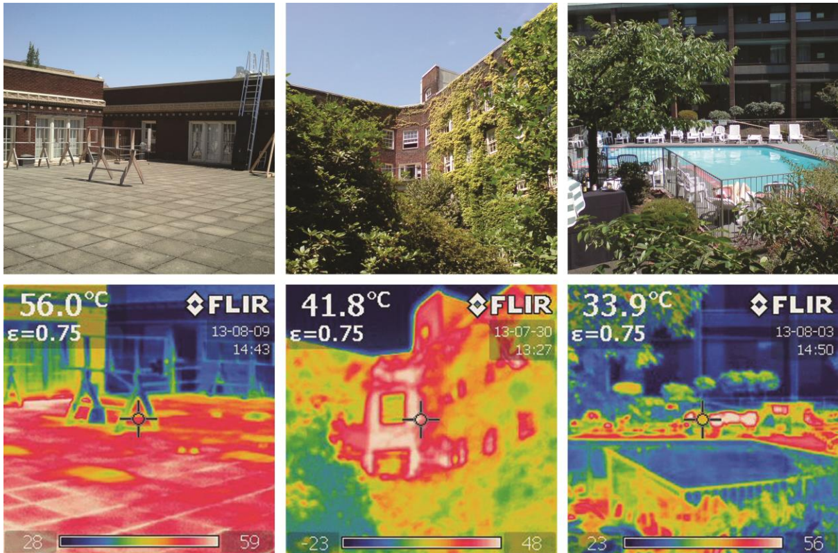
Figure 8: The three measured courtyards: bare, green and with water pool (points 3, 1 and 7, respectively in Figure 1-Phase 1).
