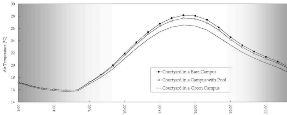
Figure 7: The air temperature of Shattuck Hall courtyard in the three campus scenarios.
