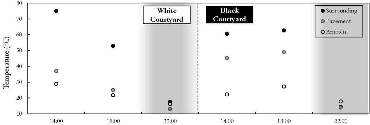
Figure 13: Temperature differences between surfaces of surrounding, white and black pavements and the ambient air.
