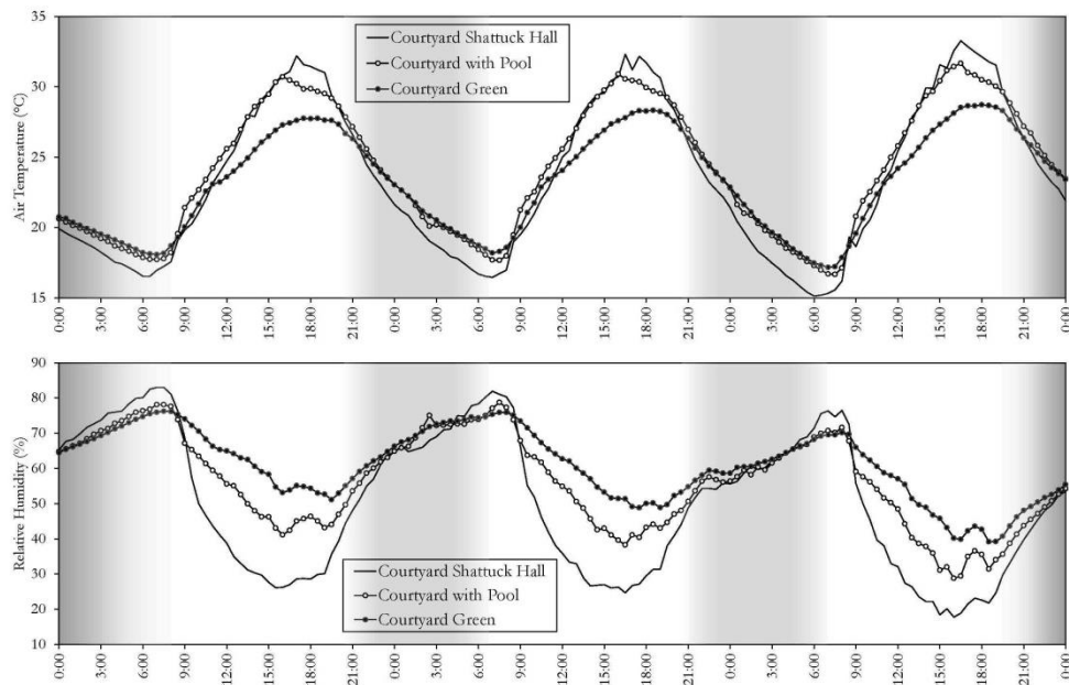
Figure 9: Air temperature and relative humidity in the measured courtyards.
