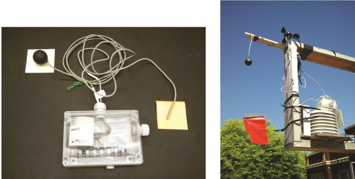
Figure 2: HOBO connected to air and globe temperature sensors (left) and in its final appearance in the field, connected to wind sensor (right).
