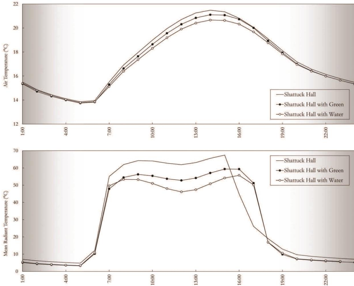
Figure 11: Air temperature (top) and mean radiant temperature (bottom) at the centre of the Shattuck hall courtyard according to the three scenarios: bare, green and with water pond.
