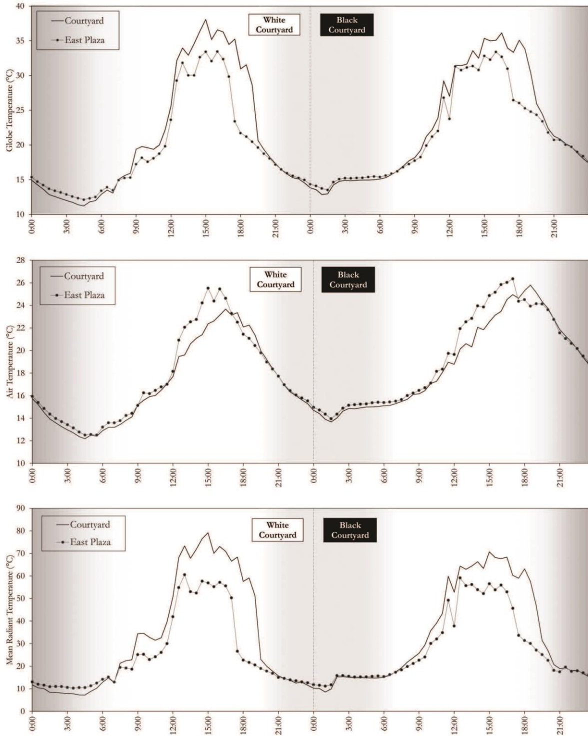
Figure 14: The globe, air and mean radiant temperature when using white and black pavements.
