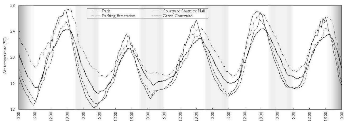
Figure 5: Temperature comparison between different locations on the campus.
