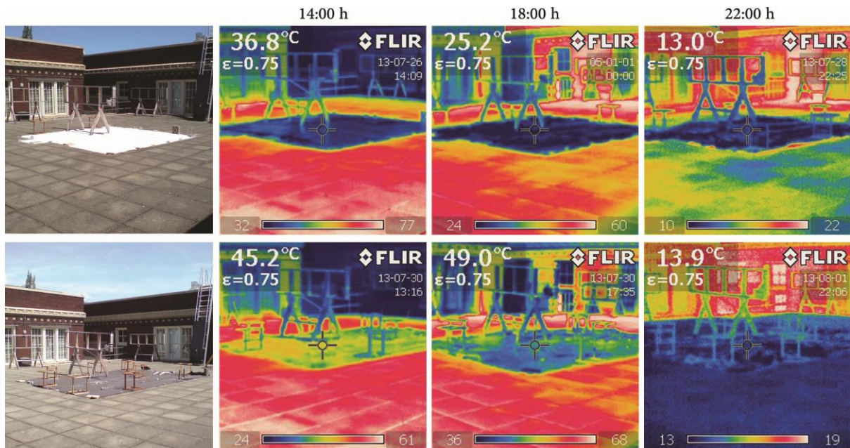
Figure 12: The effect of albedo change at different moments.
