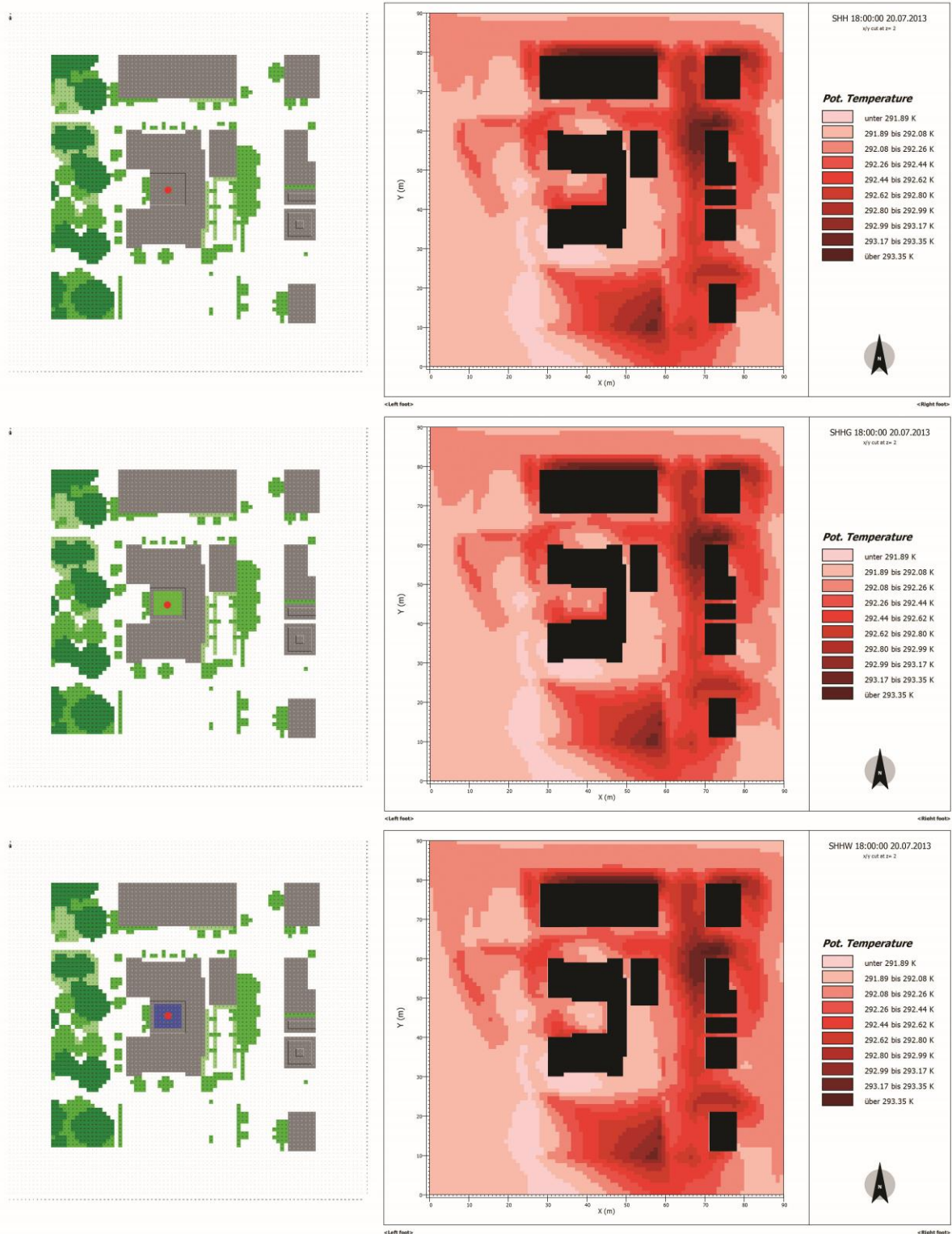
Figure 10: Air temperature in the three scenarios. Top: the bare courtyard, middle: the courtyard with grass, and bottom: the courtyard with water pond.
