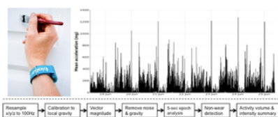
Fig 1. UK Biobank triaxial accelerometer and processing steps to extract physical activity information.
