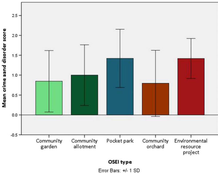
Fig. 4 Type mean crime and disorder deprivation scores. Grand mean = 1.06 \pm 0.76
