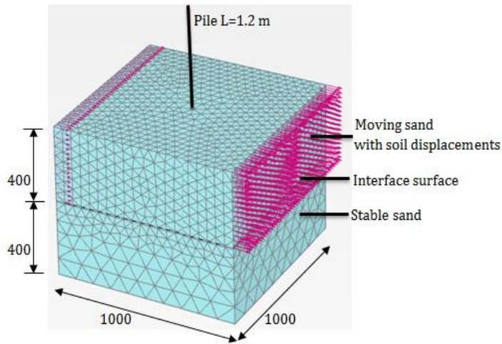
Fig. 4: Finite Element Simulation and Dimensions of the problem
