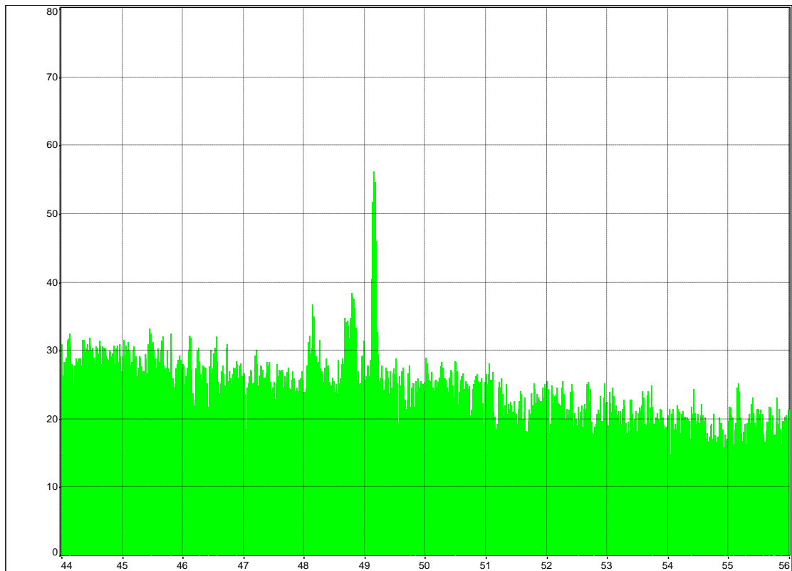
Figure 83: Zoom FFT of 9m30s of audio record starting 05h10m on 25/04/04 from measurement Case18_040424_205000.cmg showing peaks at 48.2, 48.8 and 49.2 Hz.
