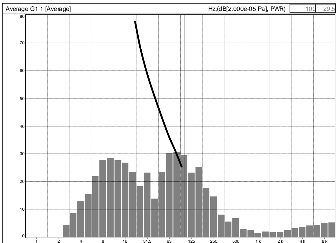
Figure 69: Mean 1/3 octave band spectrum 9m30s starting starting 02h30m on 03/04/04 from measurement Case16_040402_210000.cmg
