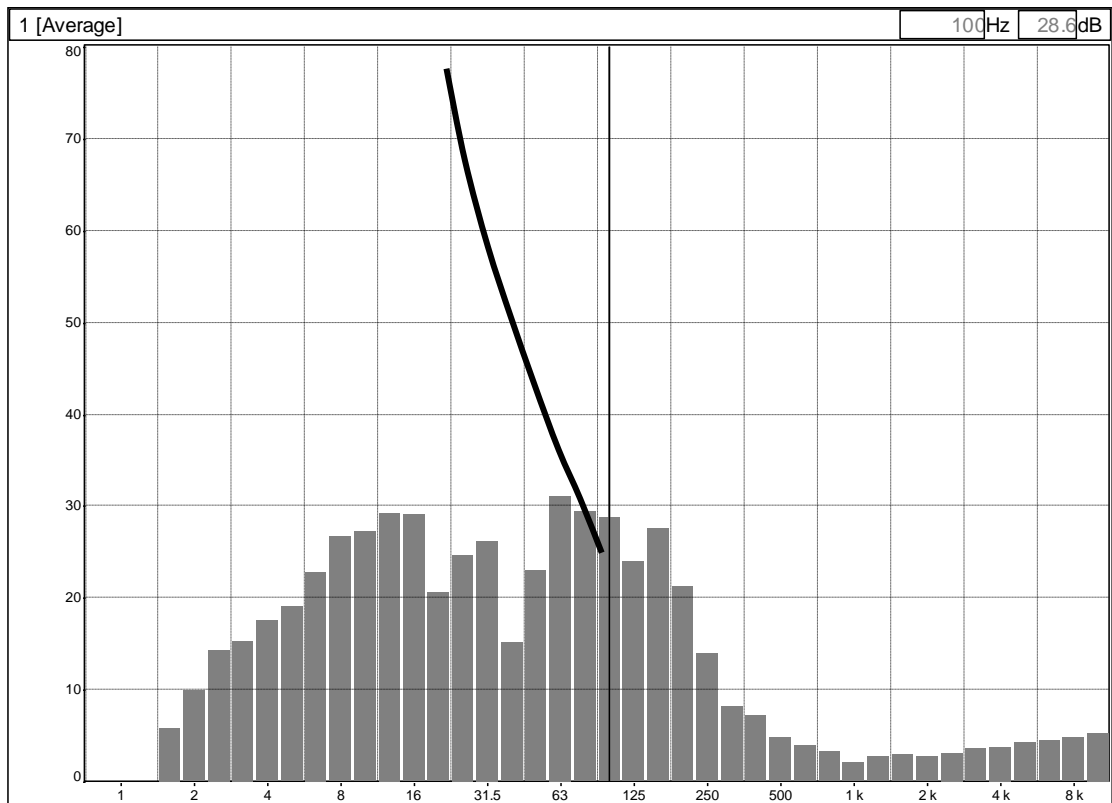
Figure 77: Mean 1/3 octave band spectrum during 2m10s of flyover starting at 02h33 on 06/04/04 from measurement Case16_040405_210000.cmg
