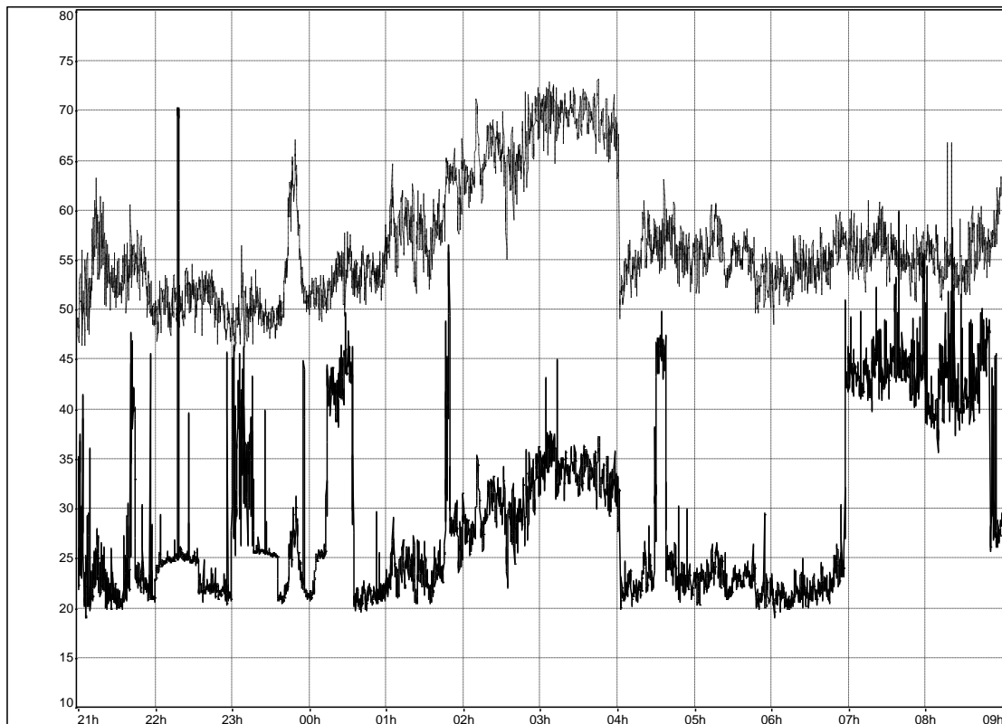
Figure 6: Time history showing 40Hz 1/3 octave spectrum band from measurement Case20_458_210000.cmg together with dBA levels. The dBA level illustrates normal household noise.
