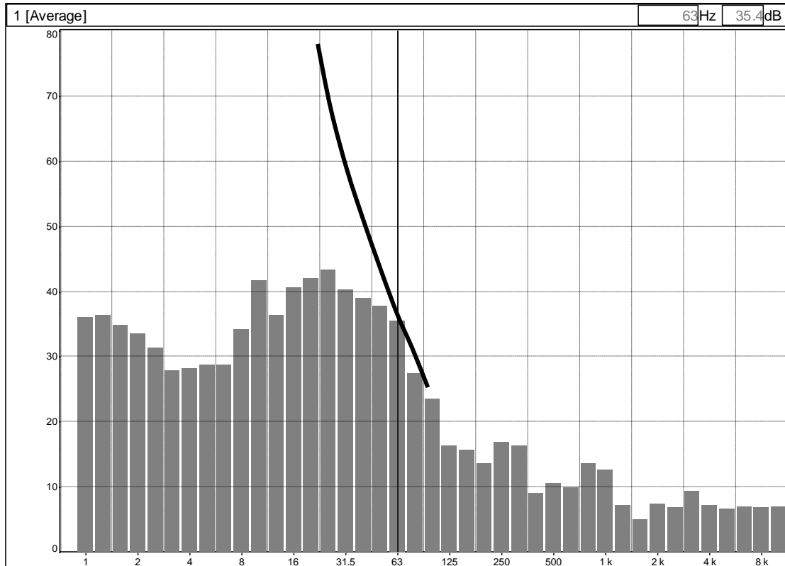
Figure 42: Mean 1/3 octave band spectrum 9m30s starting 23h20m from measurement Case5_040423_090000.cmg
