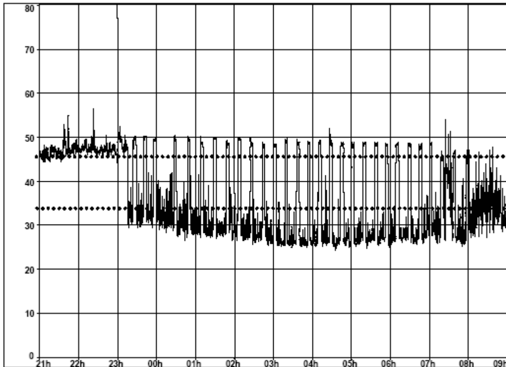
Figure 98: Time history showing 63Hz 1/3 octave spectrum band from measurement Case19a_040424_090000.cmg together with Dutch (audibility) 33dB and Danish 46.2dB limits
