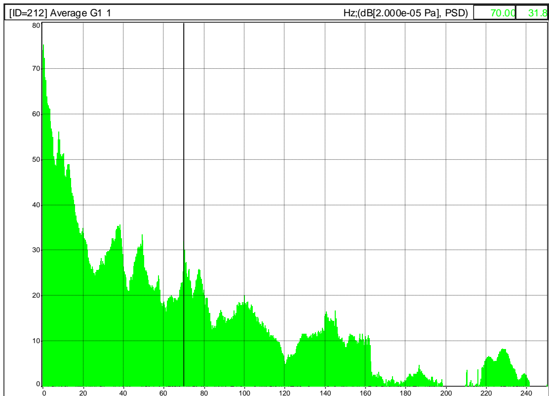
Figure 53: FFT of 9m30s audio record starting 13h30m on 15/05/04 from measurement Case7_040514_134035.cm
