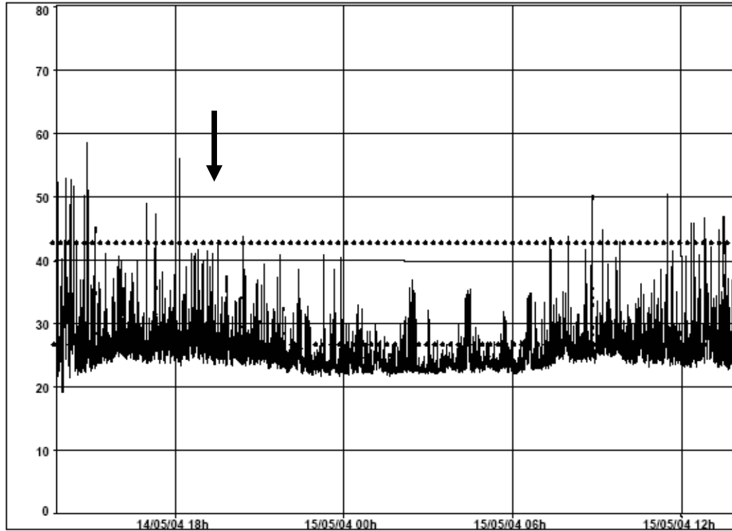
Figure 52: Time history showing 80Hz 1/3 octave spectrum band from measurement Case7_040514_134035.cm together with lower Dutch (audibility) 27dB and Danish 42.5dB limits
