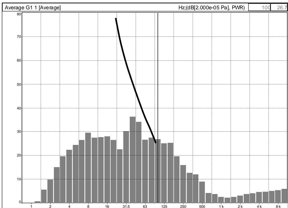
Figure 63: Mean 1/3 octave band spectrum 9m30s starting 04h00m from measurement Case13_040406_210000.cmg
