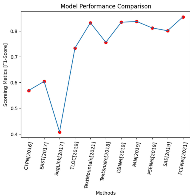
Figure 5 Detection comparison analysis over changing of time and method on CTW1500
