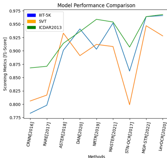
Figure 10 Detection comparison analysis over changing of time and method on regular text dataset
